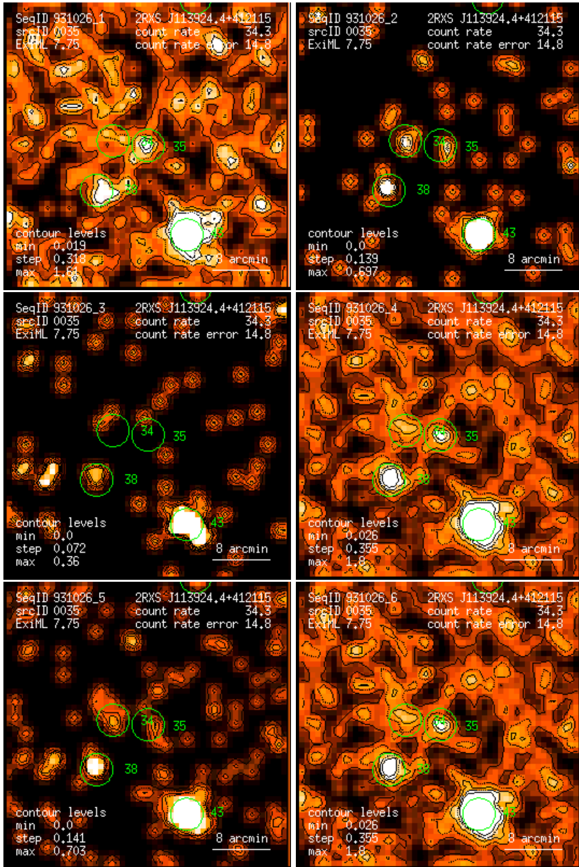
Figure 35: RASS 931026: detection 0035: band rate images, Gaussian filter: (1) PSPC channels 11 – 41, (2) 52 – 90, (3) 91 – 201, (4) 11 – 235, (5) 52 – 201, (6) 11 – 201. Broad band rates in counts/ks. Band rate contour levels in counts/ks/arcmin 2 .
