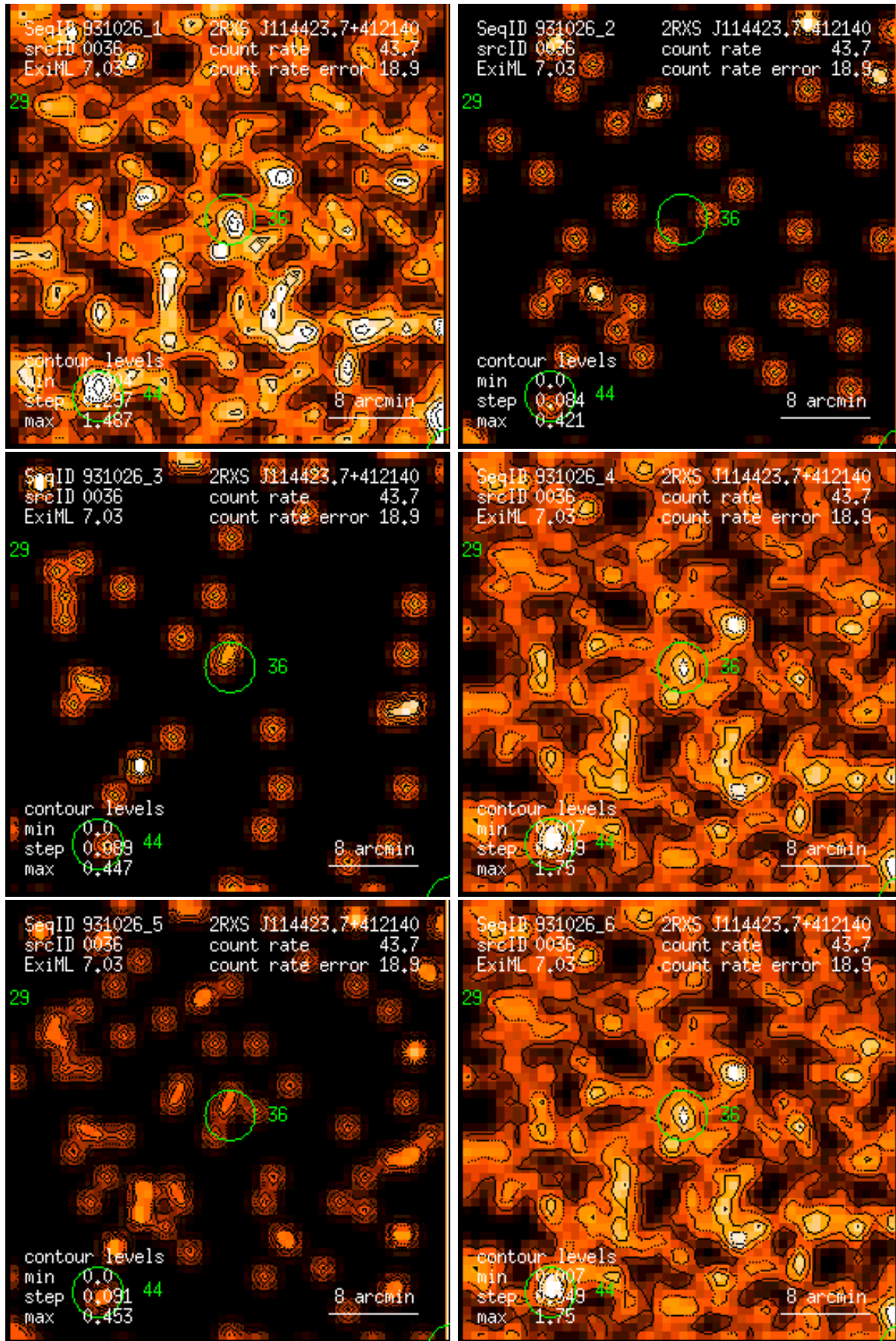
Figure 36: RASS 931026: detection 0036: band rate images, Gaussian filter: (1) PSPC channels 11 – 41, (2) 52 – 90, (3) 91 – 201, (4) 11 – 235, (5) 52 – 201, (6) 11 – 201. Broad band rates in counts/ks. Band rate contour levels in counts/ks/arcmin 2 .
