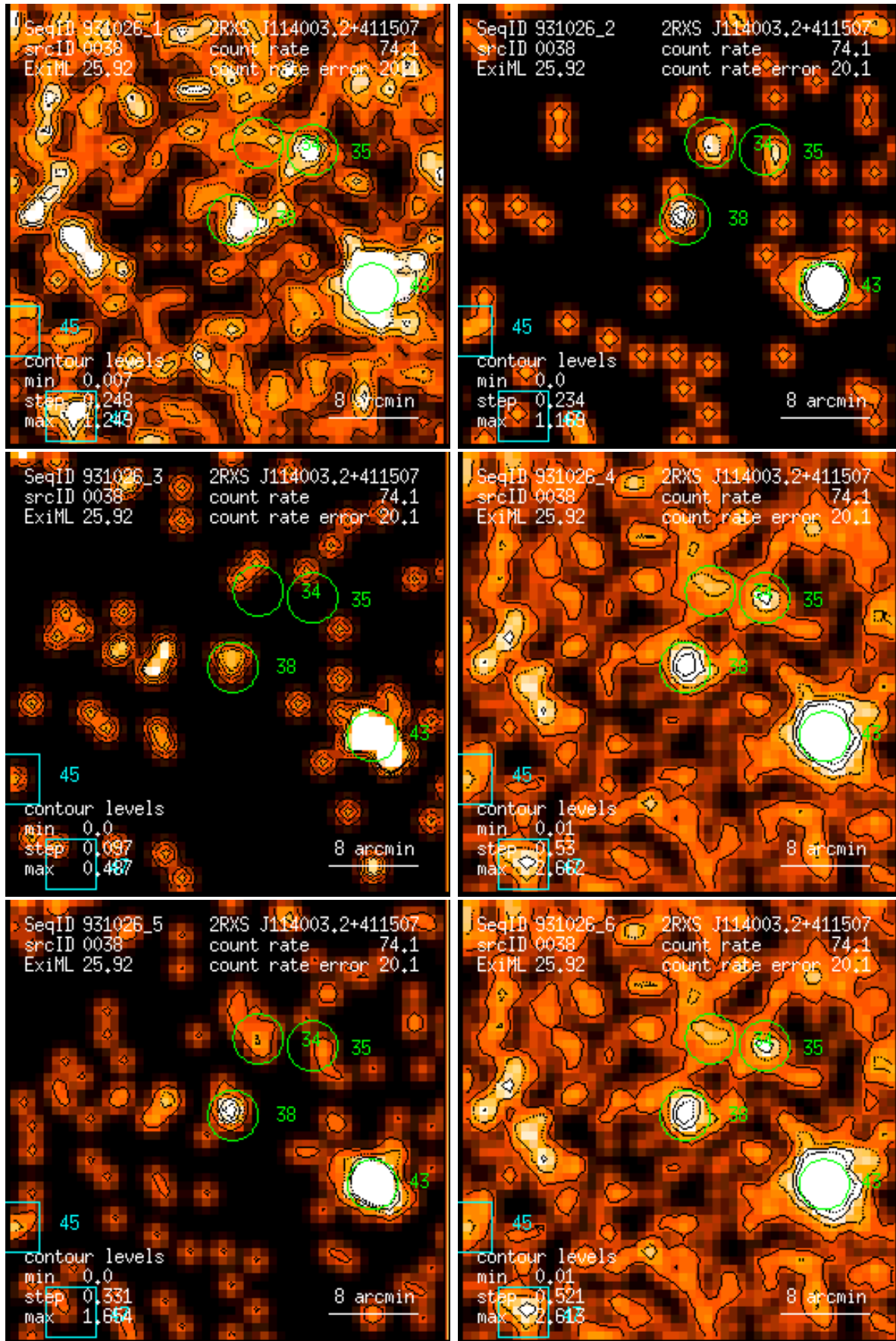
Figure 38: RASS 931026: detection 0038: band rate images, Gaussian filter: (1) PSPC channels 11 – 41, (2) 52 – 90, (3) 91 – 201, (4) 11 – 235, (5) 52 – 201, (6) 11 – 201. Broad band rates in counts/ks. Band rate contour levels in counts/ks/arcmin 2 .
