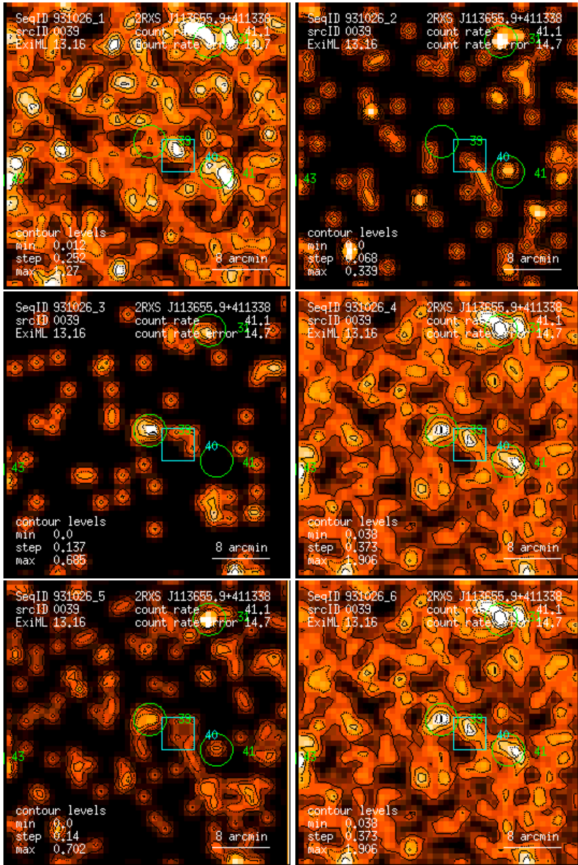
Figure 39: RASS 931026: detection 0039: band rate images, Gaussian filter: (1) PSPC channels 11 – 41, (2) 52 – 90, (3) 91 – 201, (4) 11 – 235, (5) 52 – 201, (6) 11 – 201. Broad band rates in counts/ks. Band rate contour levels in counts/ks/arcmin 2 .
