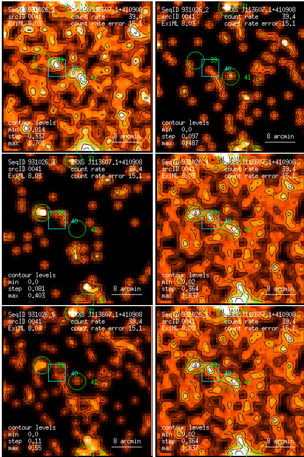
Figure 41: RASS 931026: detection 0041: band rate images, Gaussian filter: (1) PSPC channels 11 – 41, (2) 52 – 90, (3) 91 – 201, (4) 11 – 235, (5) 52 – 201, (6) 11 – 201. Broad band rates in counts/ks. Band rate contour levels in counts/ks/arcmin 2 .
