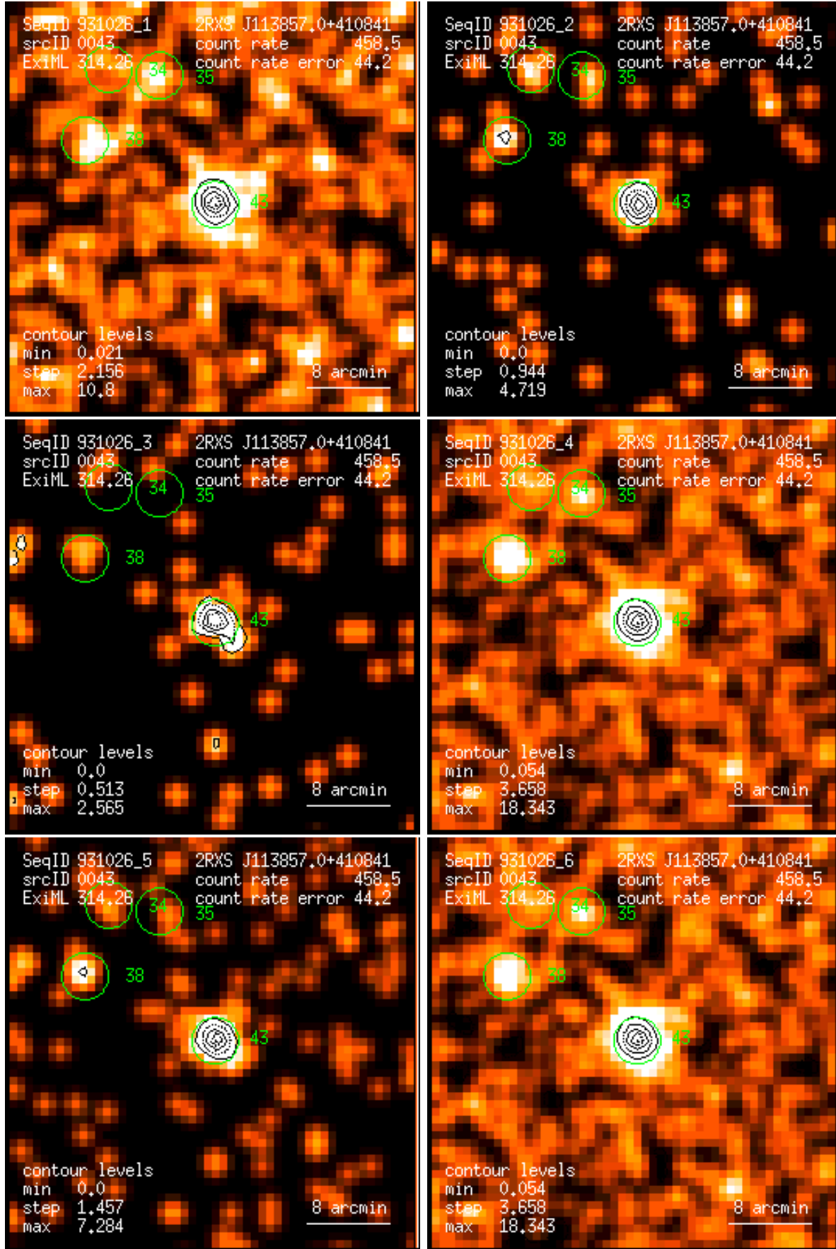
Figure 43: RASS 931026: detection 0043: band rate images, Gaussian filter: (1) PSPC channels 11 – 41, (2) 52 – 90, (3) 91 – 201, (4) 11 – 235, (5) 52 – 201, (6) 11 – 201. Broad band rates in counts/ks. Band rate contour levels in counts/ks/arcmin 2 .
