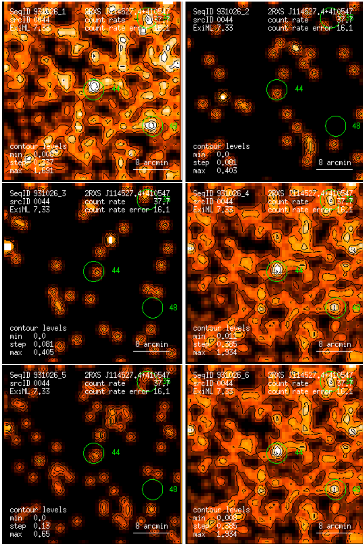
Figure 44: RASS 931026: detection 0044: band rate images, Gaussian filter: (1) PSPC channels 11 – 41, (2) 52 – 90, (3) 91 – 201, (4) 11 – 235, (5) 52 – 201, (6) 11 – 201. Broad band rates in counts/ks. Band rate contour levels in counts/ks/arcmin 2 .
