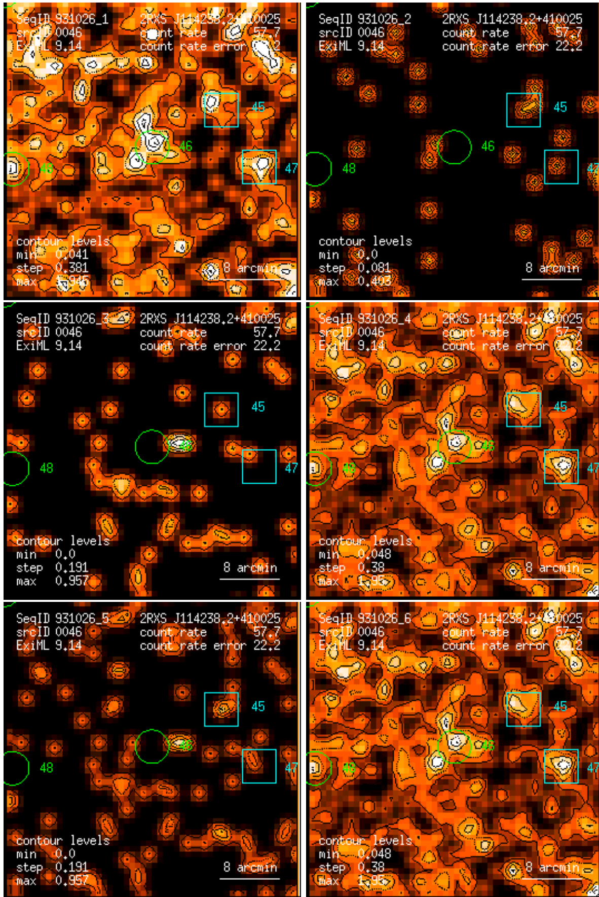
Figure 46: RASS 931026: detection 0046: band rate images, Gaussian filter: (1) PSPC channels 11 – 41, (2) 52 – 90, (3) 91 – 201, (4) 11 – 235, (5) 52 – 201, (6) 11 – 201. Broad band rates in counts/ks. Band rate contour levels in counts/ks/arcmin 2 .
