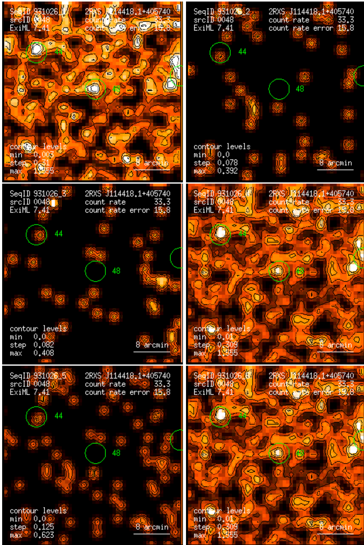
Figure 48: RASS 931026: detection 0048: band rate images, Gaussian filter: (1) PSPC channels 11 – 41, (2) 52 – 90, (3) 91 – 201, (4) 11 – 235, (5) 52 – 201, (6) 11 – 201. Broad band rates in counts/ks. Band rate contour levels in counts/ks/arcmin 2 .
