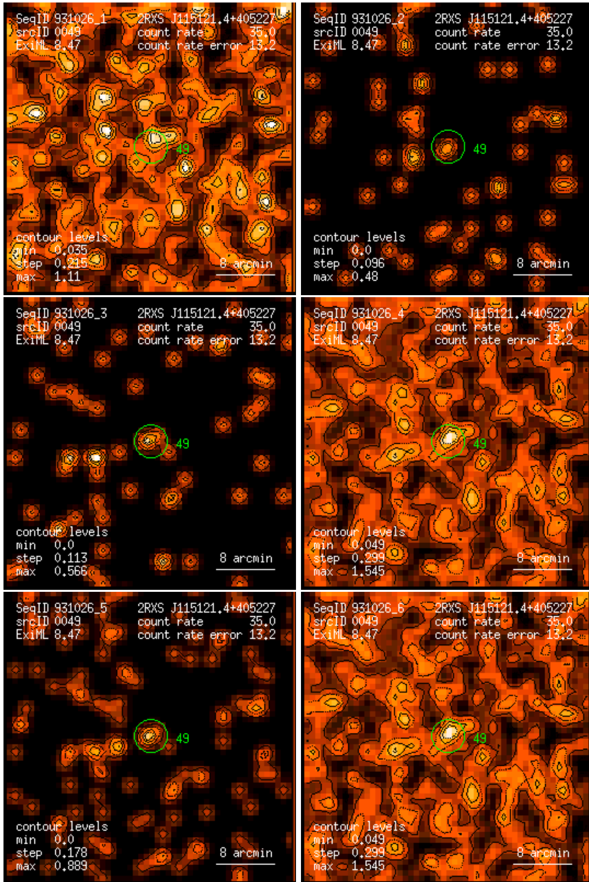
Figure 49: RASS 931026: detection 0049: band rate images, Gaussian filter: (1) PSPC channels 11 – 41, (2) 52 – 90, (3) 91 – 201, (4) 11 – 235, (5) 52 – 201, (6) 11 – 201. Broad band rates in counts/ks. Band rate contour levels in counts/ks/arcmin 2 .
