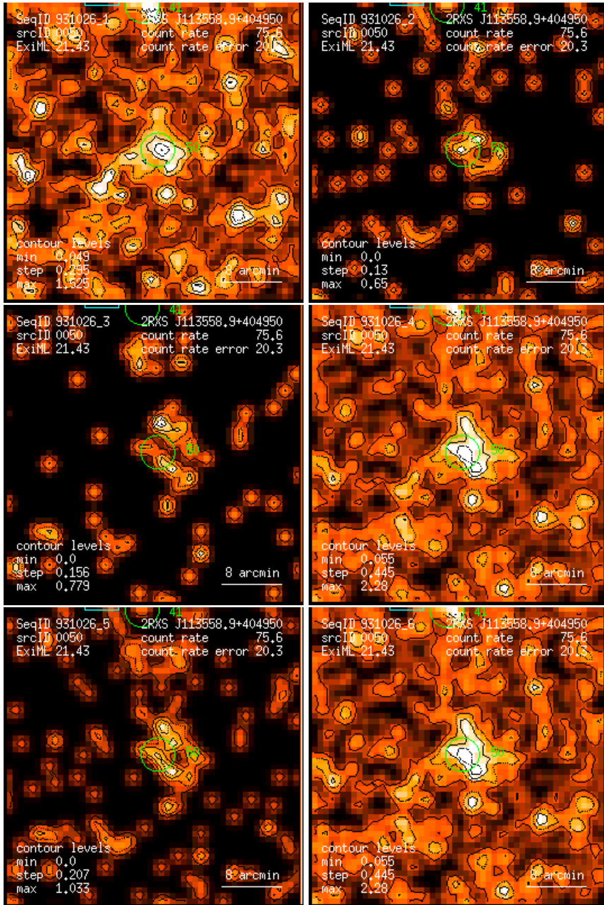
Figure 50: RASS 931026: detection 0050: band rate images, Gaussian filter: (1) PSPC channels 11 – 41, (2) 52 – 90, (3) 91 – 201, (4) 11 – 235, (5) 52 – 201, (6) 11 – 201. Broad band rates in counts/ks. Band rate contour levels in counts/ks/arcmin 2 .
