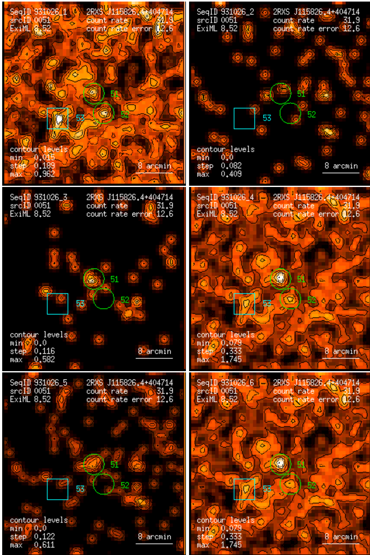
Figure 51: RASS 931026: detection 0051: band rate images, Gaussian filter: (1) PSPC channels 11 – 41, (2) 52 – 90, (3) 91 – 201, (4) 11 – 235, (5) 52 – 201, (6) 11 – 201. Broad band rates in counts/ks. Band rate contour levels in counts/ks/arcmin 2 .
