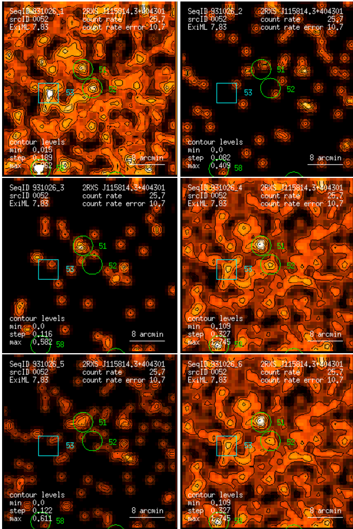
Figure 52: RASS 931026: detection 0052: band rate images, Gaussian filter: (1) PSPC channels 11 – 41, (2) 52 – 90, (3) 91 – 201, (4) 11 – 235, (5) 52 – 201, (6) 11 – 201. Broad band rates in counts/ks. Band rate contour levels in counts/ks/arcmin 2 .
