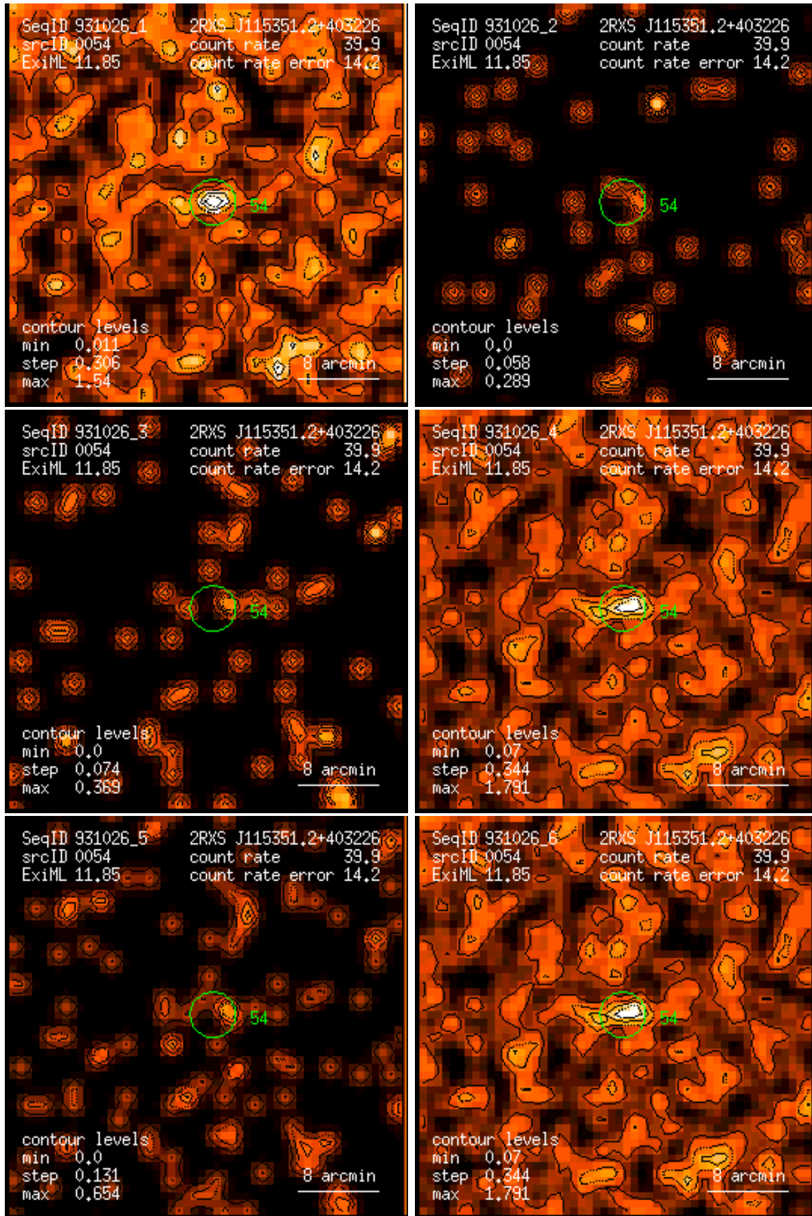
Figure 54: RASS 931026: detection 0054: band rate images, Gaussian filter: (1) PSPC channels 11 – 41, (2) 52 – 90, (3) 91 – 201, (4) 11 – 235, (5) 52 – 201, (6) 11 – 201. Broad band rates in counts/ks. Band rate contour levels in counts/ks/arcmin 2 .
