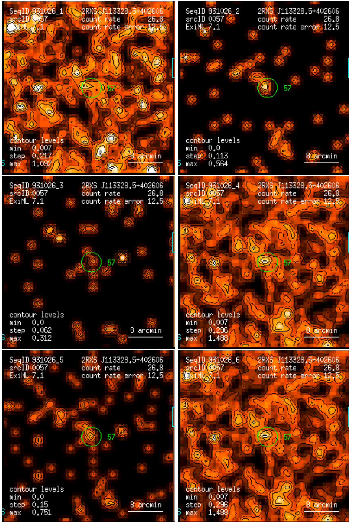
Figure 57: RASS 931026: detection 0057: band rate images, Gaussian filter: (1) PSPC channels 11 – 41, (2) 52 – 90, (3) 91 – 201, (4) 11 – 235, (5) 52 – 201, (6) 11 – 201. Broad band rates in counts/ks. Band rate contour levels in counts/ks/arcmin 2 .
