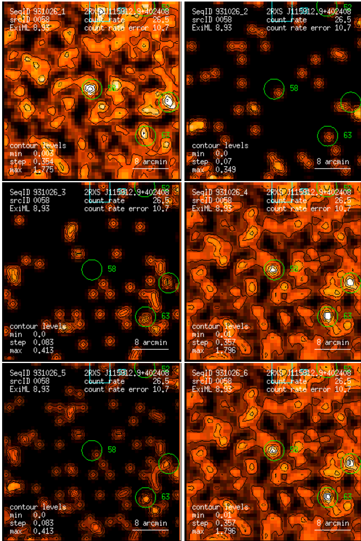
Figure 58: RASS 931026: detection 0058: band rate images, Gaussian filter: (1) PSPC channels 11 – 41, (2) 52 – 90, (3) 91 – 201, (4) 11 – 235, (5) 52 – 201, (6) 11 – 201. Broad band rates in counts/ks. Band rate contour levels in counts/ks/arcmin 2 .
