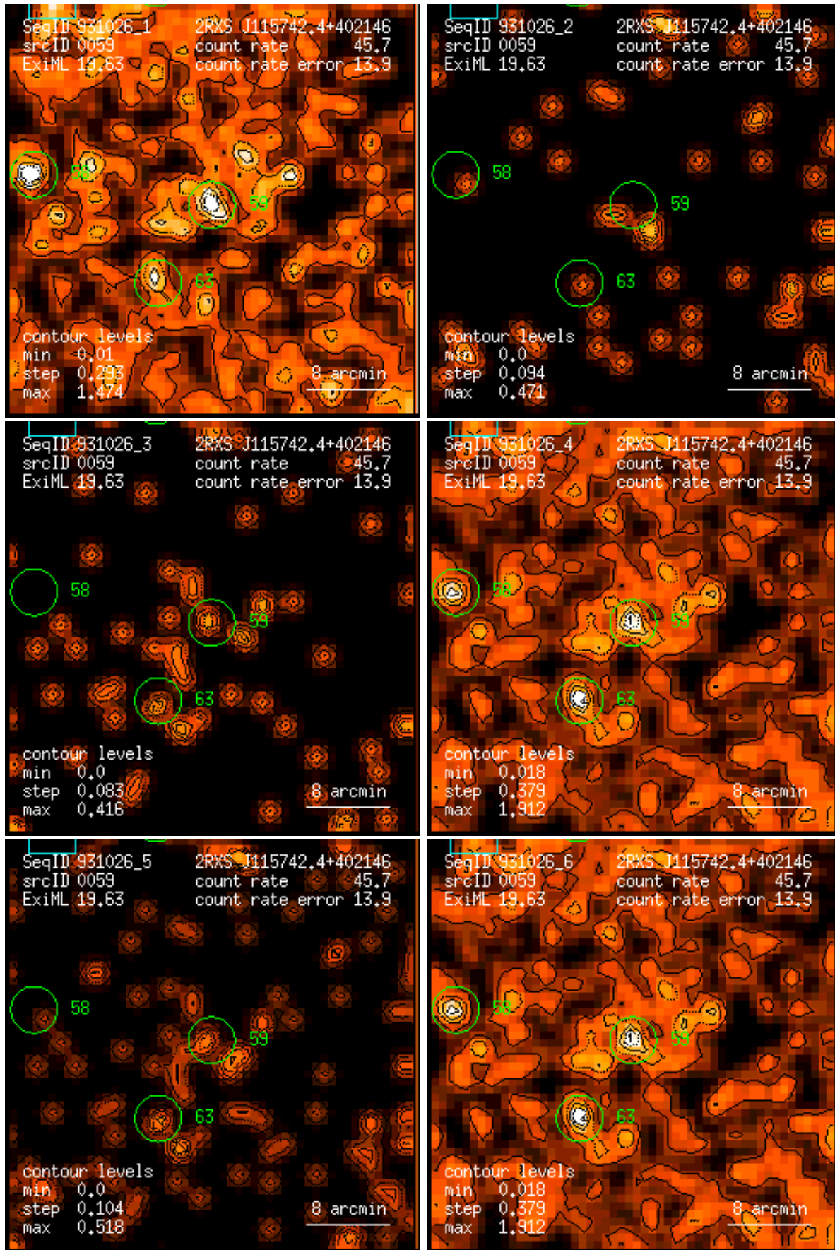
Figure 59: RASS 931026: detection 0059: band rate images, Gaussian filter: (1) PSPC channels 11 – 41, (2) 52 – 90, (3) 91 – 201, (4) 11 – 235, (5) 52 – 201, (6) 11 – 201. Broad band rates in counts/ks. Band rate contour levels in counts/ks/arcmin 2 .
