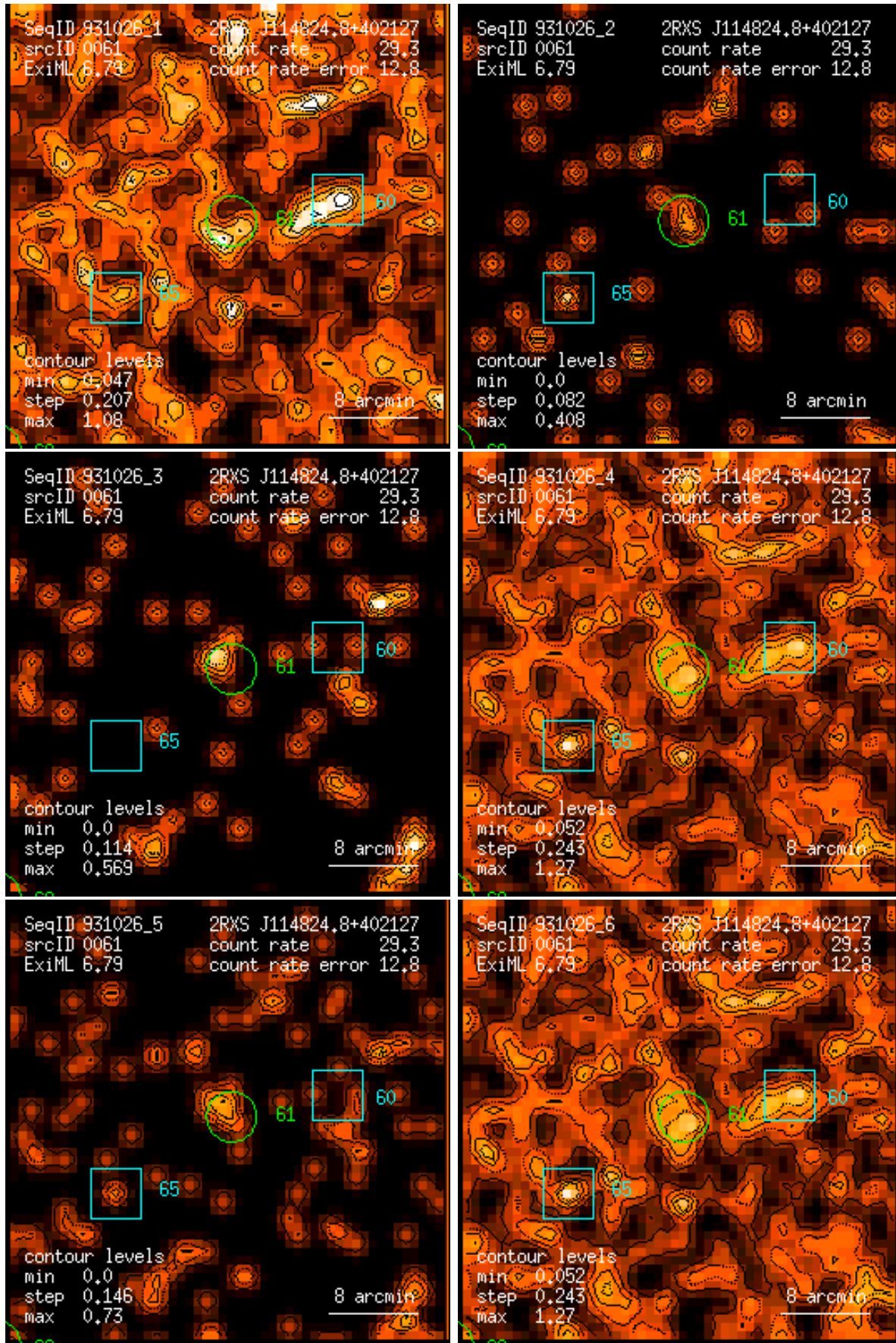
Figure 61: RASS 931026: detection 0061: band rate images, Gaussian filter: (1) PSPC channels 11 – 41, (2) 52 – 90, (3) 91 – 201, (4) 11 – 235, (5) 52 – 201, (6) 11 – 201. Broad band rates in counts/ks. Band rate contour levels in counts/ks/arcmin 2 .
