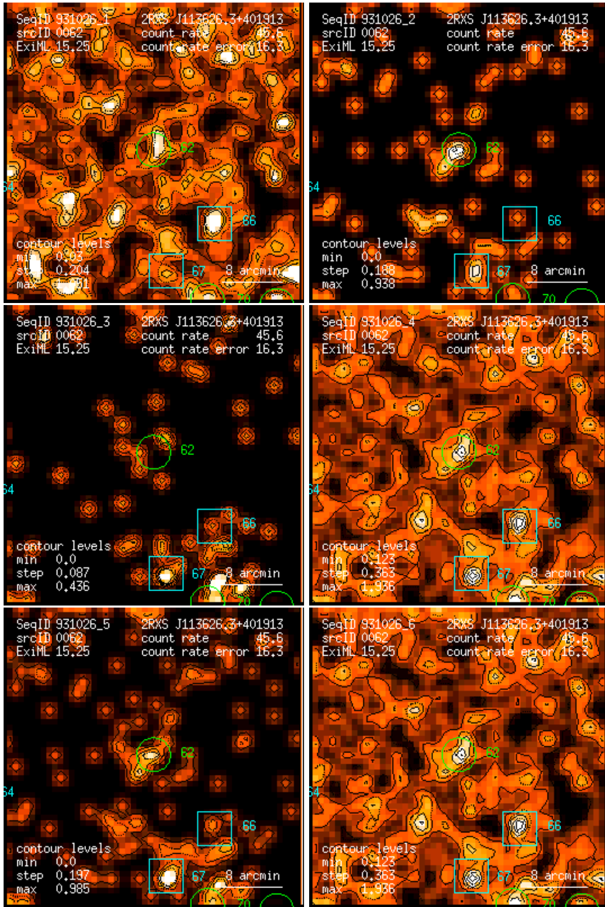
Figure 62: RASS 931026: detection 0062: band rate images, Gaussian filter: (1) PSPC channels 11 – 41, (2) 52 – 90, (3) 91 – 201, (4) 11 – 235, (5) 52 – 201, (6) 11 – 201. Broad band rates in counts/ks. Band rate contour levels in counts/ks/arcmin 2 .
