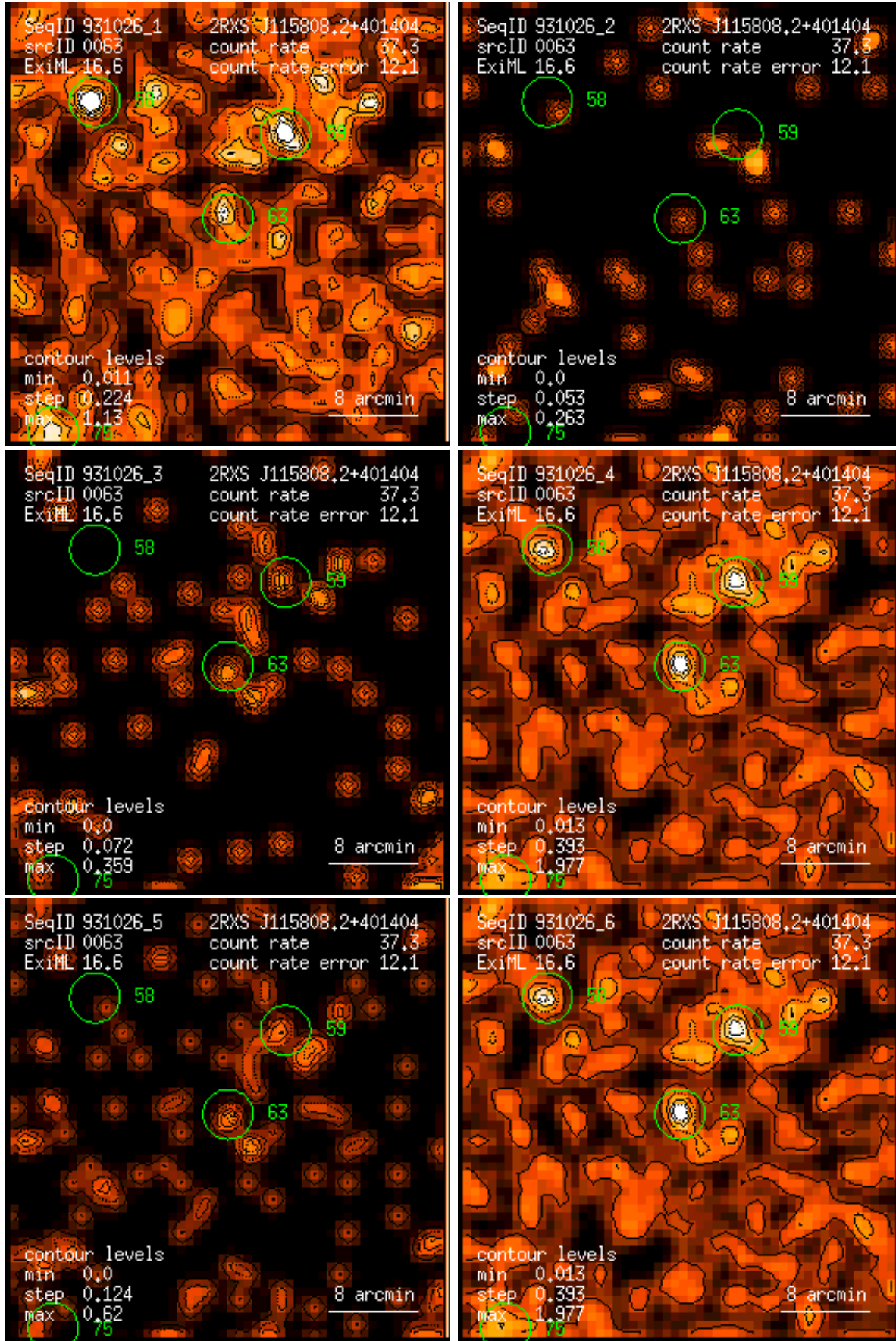
Figure 63: RASS 931026: detection 0063: band rate images, Gaussian filter: (1) PSPC channels 11 – 41, (2) 52 – 90, (3) 91 – 201, (4) 11 – 235, (5) 52 – 201, (6) 11 – 201. Broad band rates in counts/ks. Band rate contour levels in counts/ks/arcmin 2 .
