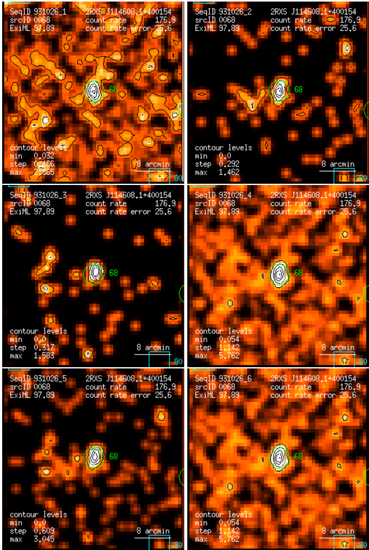
Figure 68: RASS 931026: detection 0068: band rate images, Gaussian filter: (1) PSPC channels 11 – 41, (2) 52 – 90, (3) 91 – 201, (4) 11 – 235, (5) 52 – 201, (6) 11 – 201. Broad band rates in counts/ks. Band rate contour levels in counts/ks/arcmin 2 .
