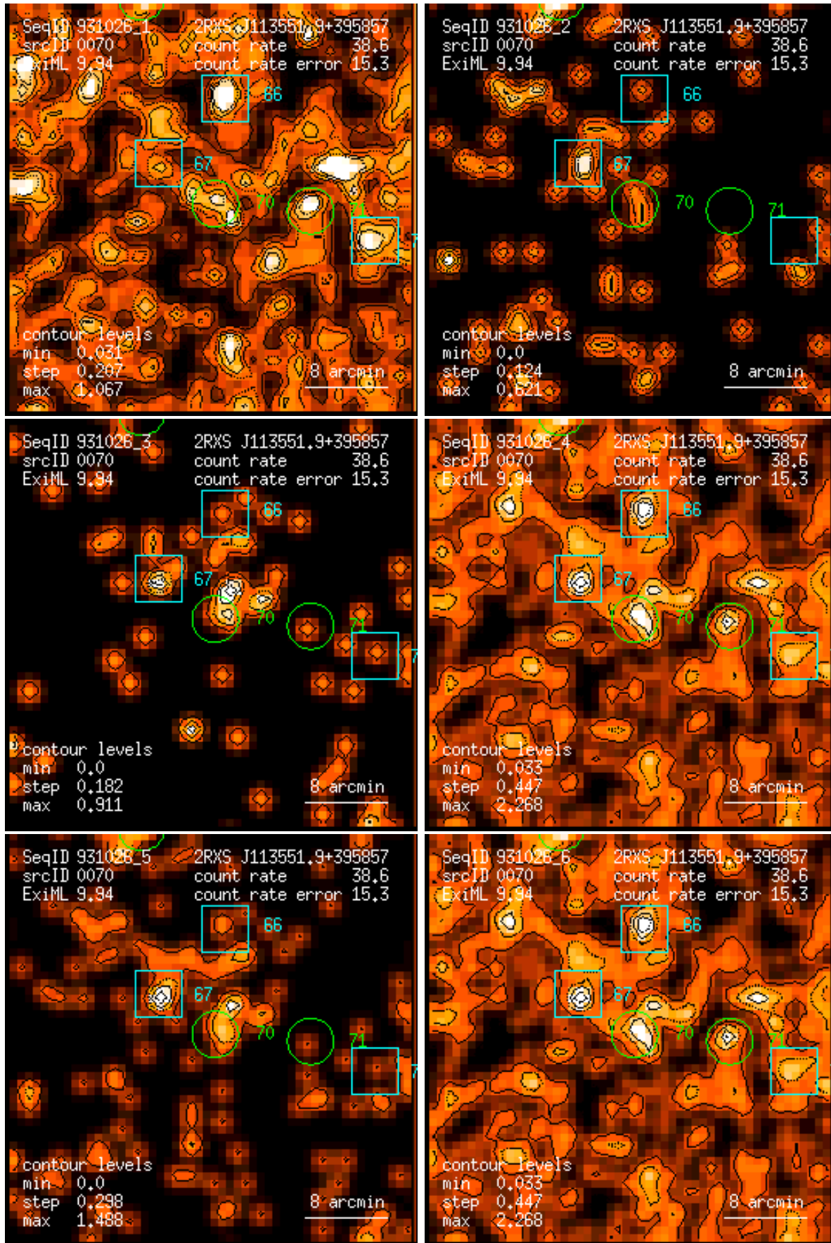
Figure 70: RASS 931026: detection 0070: band rate images, Gaussian filter: (1) PSPC channels 11 – 41, (2) 52 – 90, (3) 91 – 201, (4) 11 – 235, (5) 52 – 201, (6) 11 – 201. Broad band rates in counts/ks. Band rate contour levels in counts/ks/arcmin 2 .
