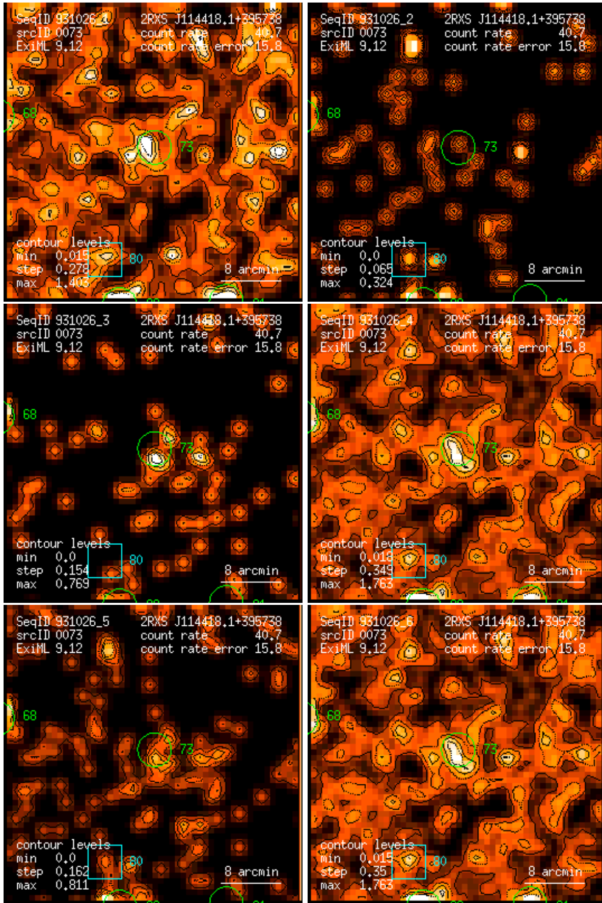
Figure 73: RASS 931026: detection 0073: band rate images, Gaussian filter: (1) PSPC channels 11 – 41, (2) 52 – 90, (3) 91 – 201, (4) 11 – 235, (5) 52 – 201, (6) 11 – 201. Broad band rates in counts/ks. Band rate contour levels in counts/ks/arcmin 2 .
