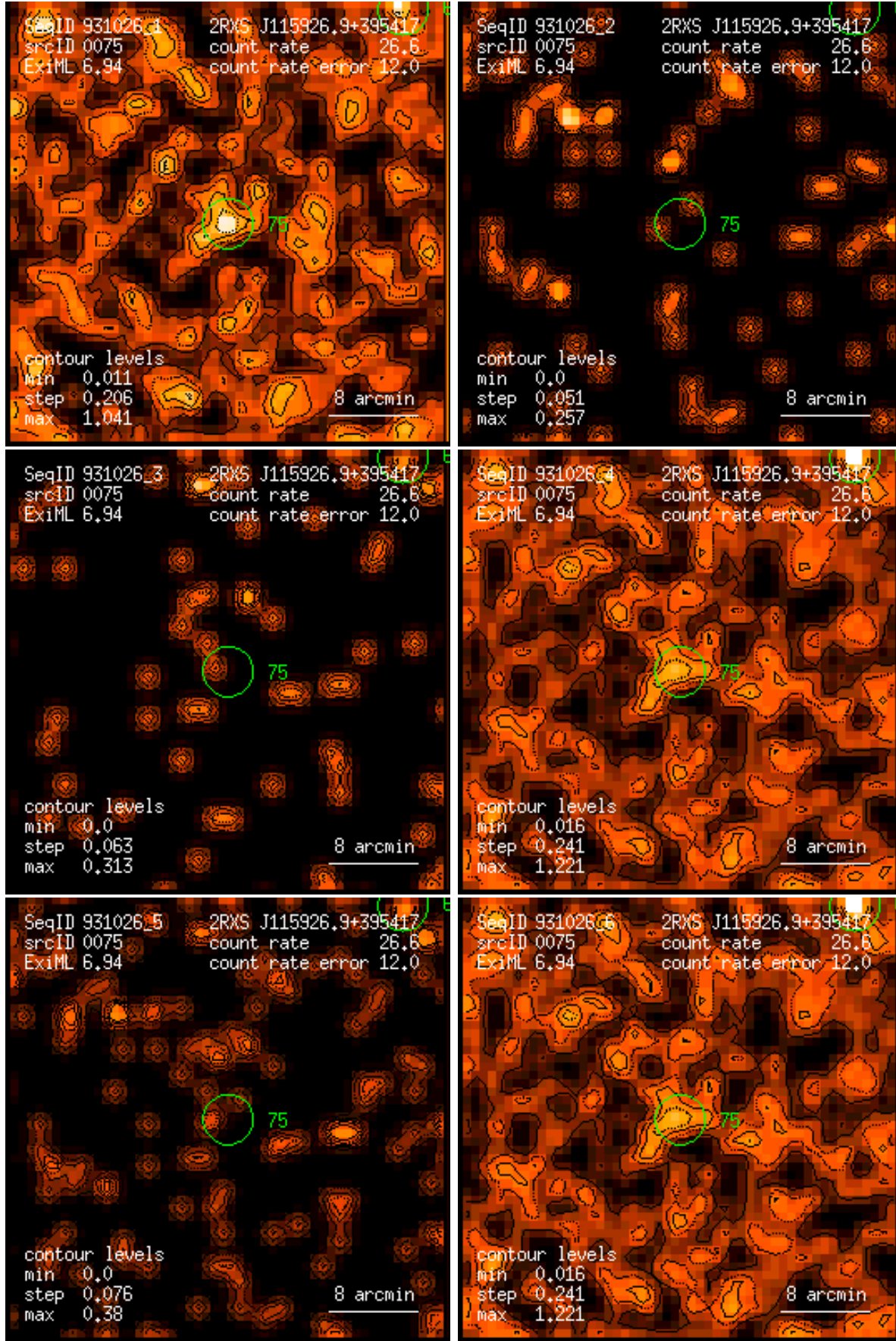
Figure 75: RASS 931026: detection 0075: band rate images, Gaussian filter: (1) PSPC channels 11 – 41, (2) 52 – 90, (3) 91 – 201, (4) 11 – 235, (5) 52 – 201, (6) 11 – 201. Broad band rates in counts/ks. Band rate contour levels in counts/ks/arcmin 2 .
