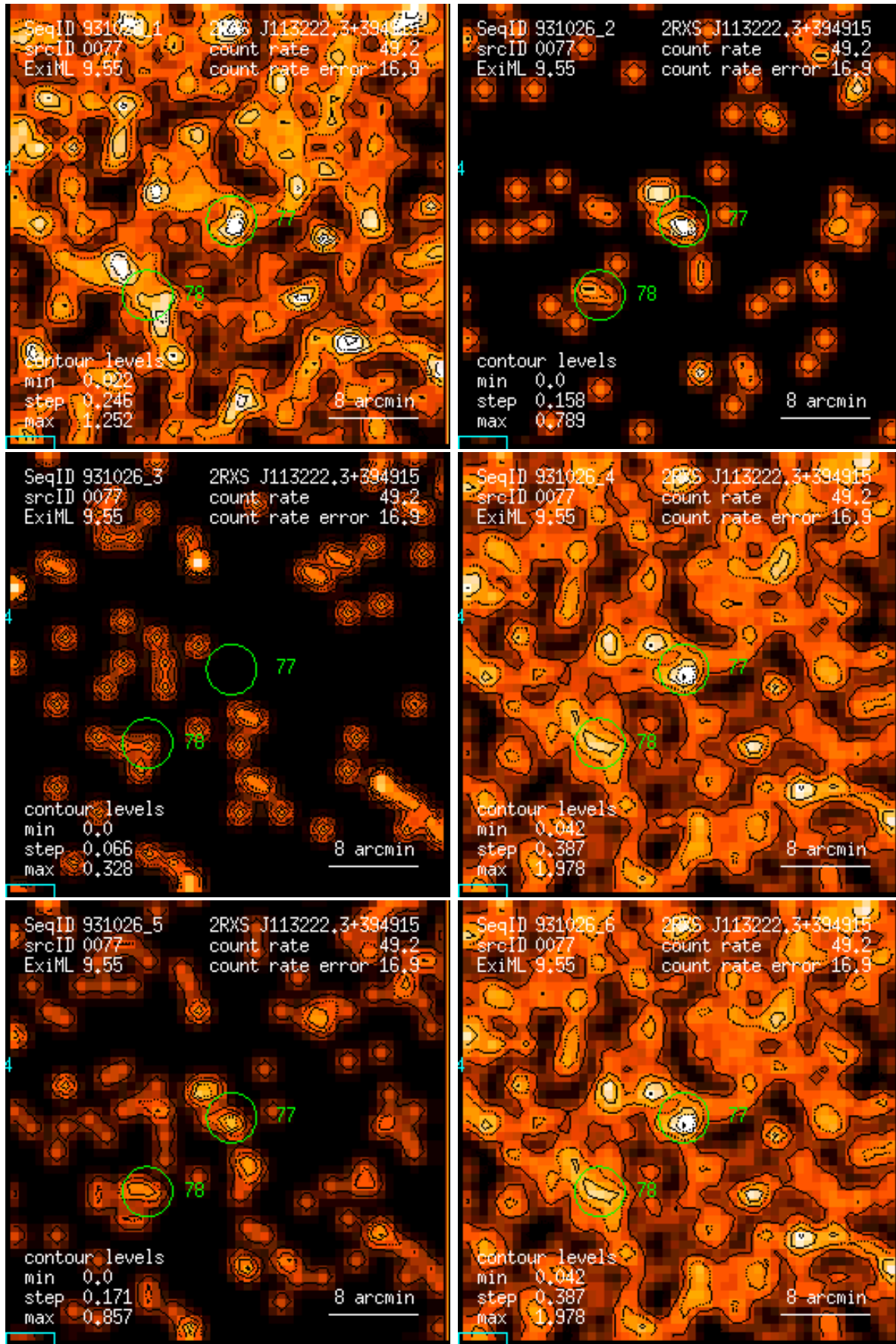
Figure 77: RASS 931026: detection 0077: band rate images, Gaussian filter: (1) PSPC channels 11 – 41, (2) 52 – 90, (3) 91 – 201, (4) 11 – 235, (5) 52 – 201, (6) 11 – 201. Broad band rates in counts/ks. Band rate contour levels in counts/ks/arcmin 2 .
