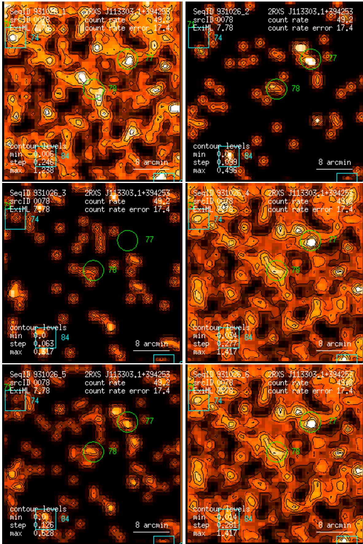
Figure 78: RASS 931026: detection 0078: band rate images, Gaussian filter: (1) PSPC channels 11 – 41, (2) 52 – 90, (3) 91 – 201, (4) 11 – 235, (5) 52 – 201, (6) 11 – 201. Broad band rates in counts/ks. Band rate contour levels in counts/ks/arcmin 2 .
