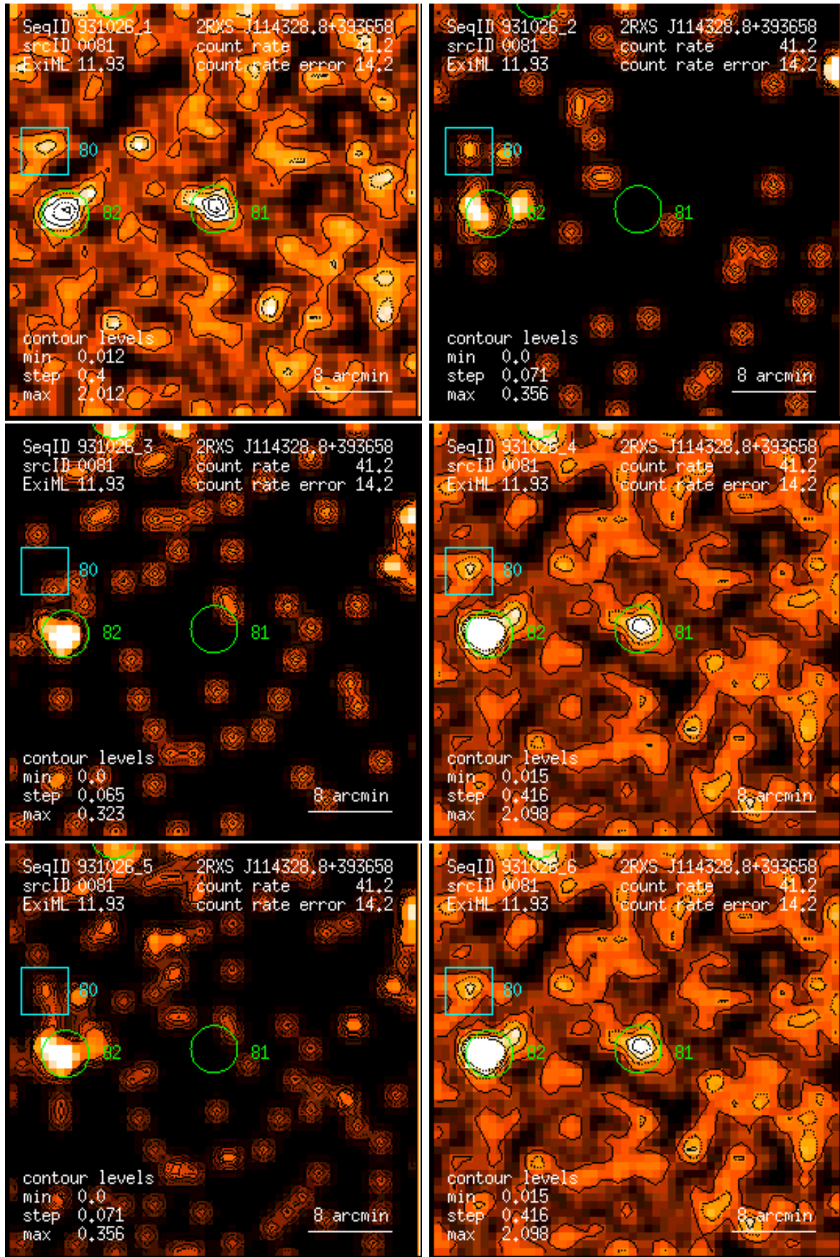
Figure 81: RASS 931026: detection 0081: band rate images, Gaussian filter: (1) PSPC channels 11 – 41, (2) 52 – 90, (3) 91 – 201, (4) 11 – 235, (5) 52 – 201, (6) 11 – 201. Broad band rates in counts/ks. Band rate contour levels in counts/ks/arcmin 2 .
