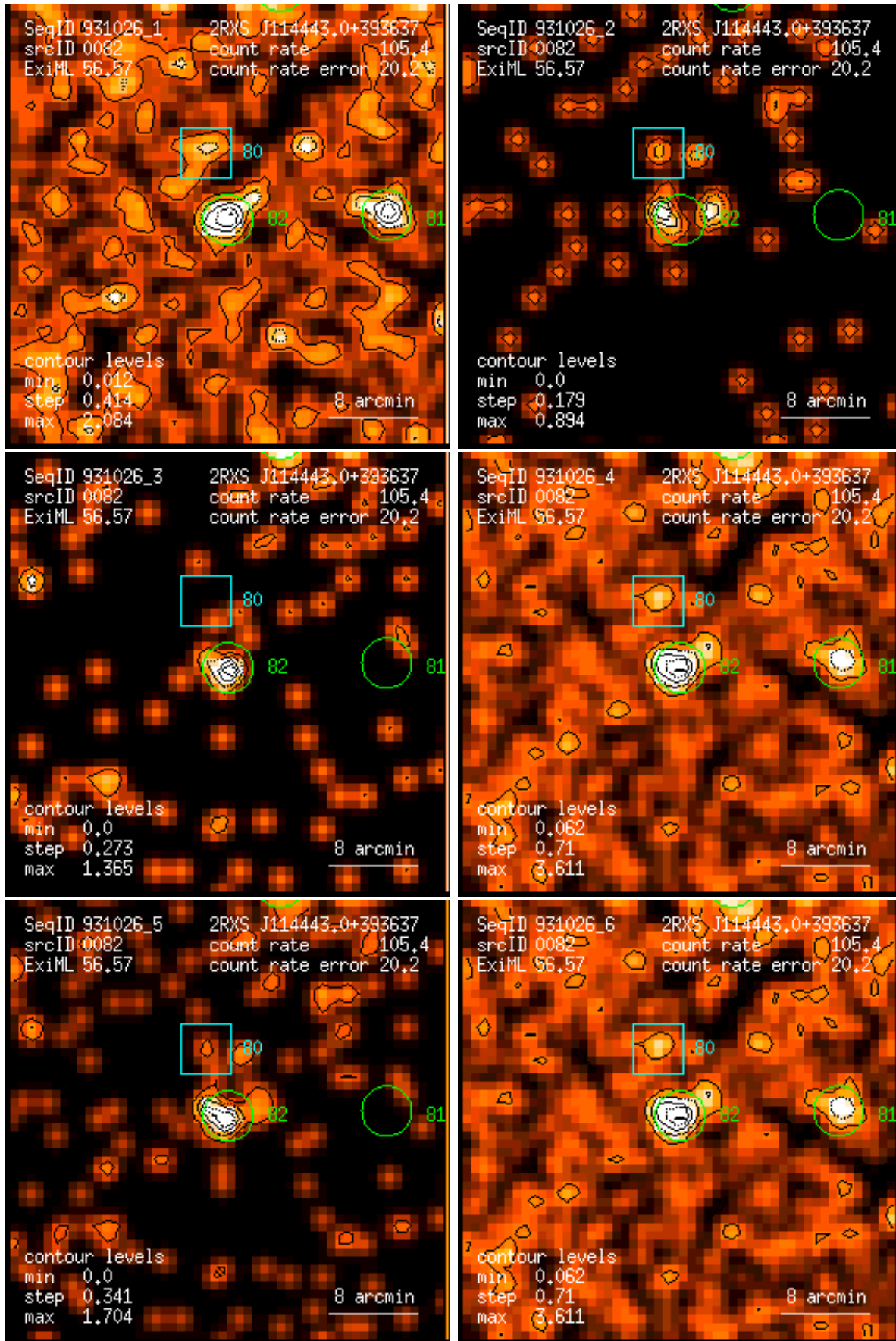
Figure 82: RASS 931026: detection 0082: band rate images, Gaussian filter: (1) PSPC channels 11 – 41, (2) 52 – 90, (3) 91 – 201, (4) 11 – 235, (5) 52 – 201, (6) 11 – 201. Broad band rates in counts/ks. Band rate contour levels in counts/ks/arcmin 2 .
