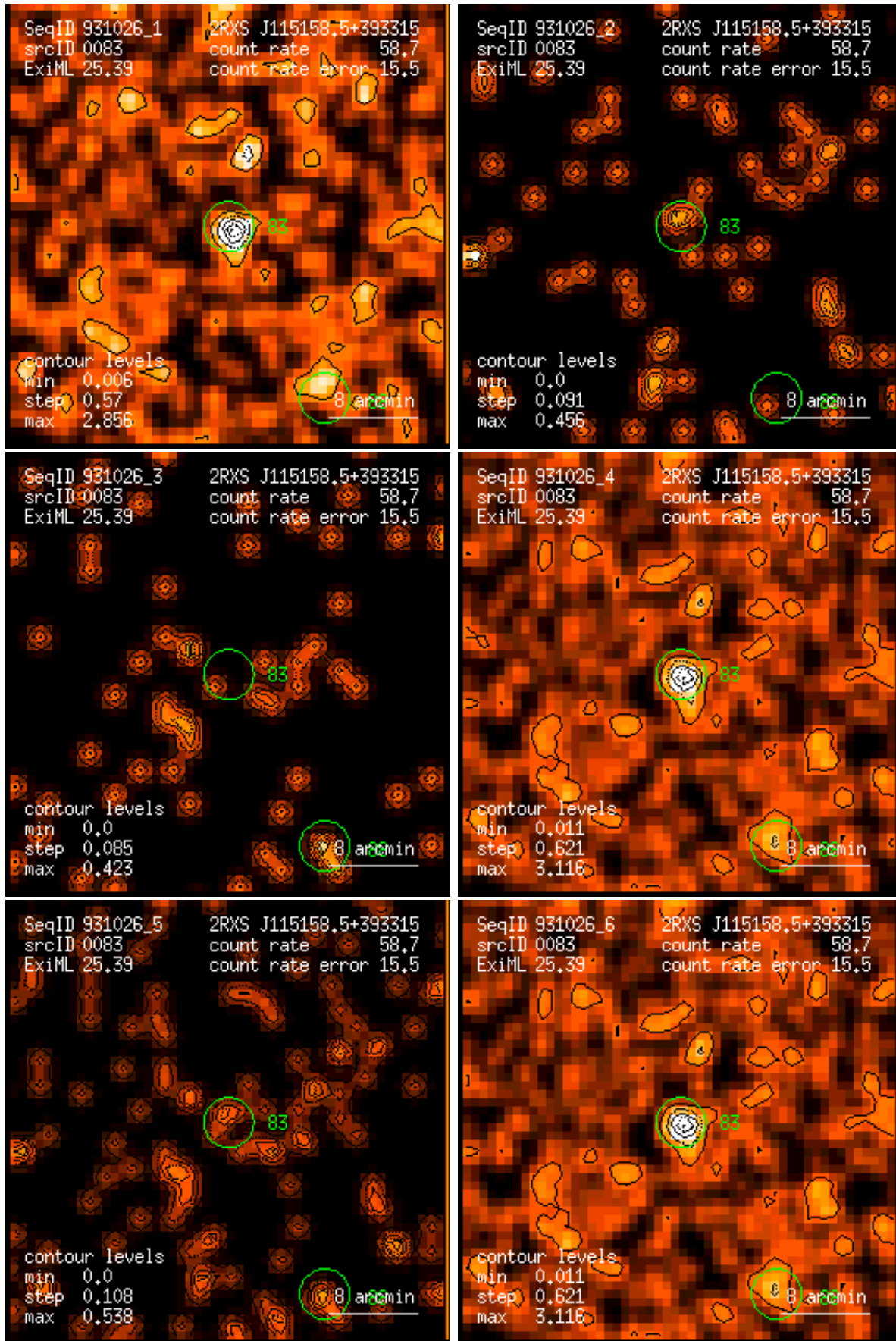
Figure 83: RASS 931026: detection 0083: band rate images, Gaussian filter: (1) PSPC channels 11 – 41, (2) 52 – 90, (3) 91 – 201, (4) 11 – 235, (5) 52 – 201, (6) 11 – 201. Broad band rates in counts/ks. Band rate contour levels in counts/ks/arcmin 2 .
