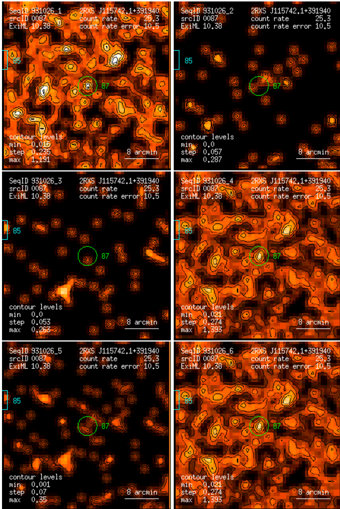
Figure 87: RASS 931026: detection 0087: band rate images, Gaussian filter: (1) PSPC channels 11 – 41, (2) 52 – 90, (3) 91 – 201, (4) 11 – 235, (5) 52 – 201, (6) 11 – 201. Broad band rates in counts/ks. Band rate contour levels in counts/ks/arcmin 2 .
