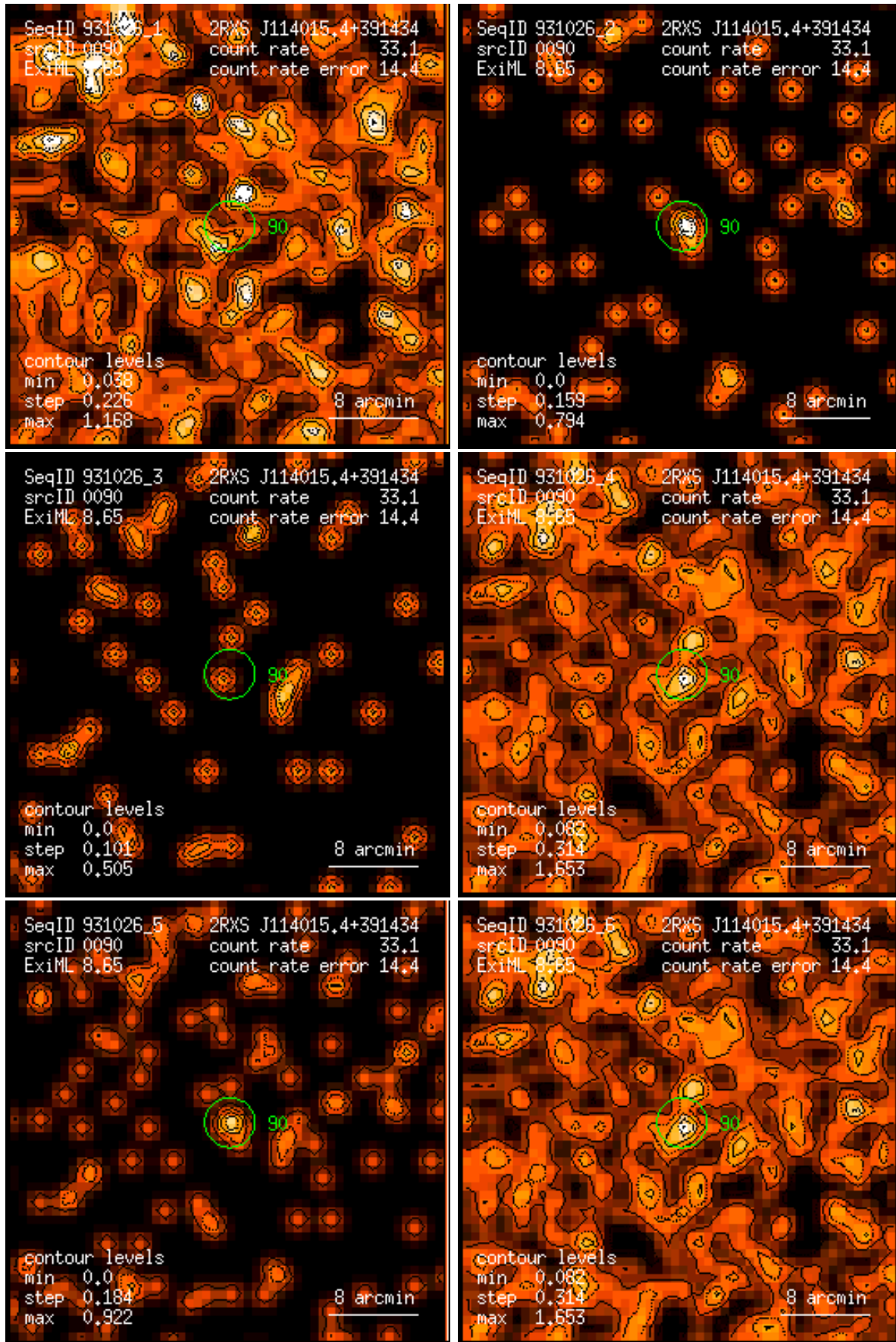
Figure 90: RASS 931026: detection 0090: band rate images, Gaussian filter: (1) PSPC channels 11 – 41, (2) 52 – 90, (3) 91 – 201, (4) 11 – 235, (5) 52 – 201, (6) 11 – 201. Broad band rates in counts/ks. Band rate contour levels in counts/ks/arcmin 2 .
