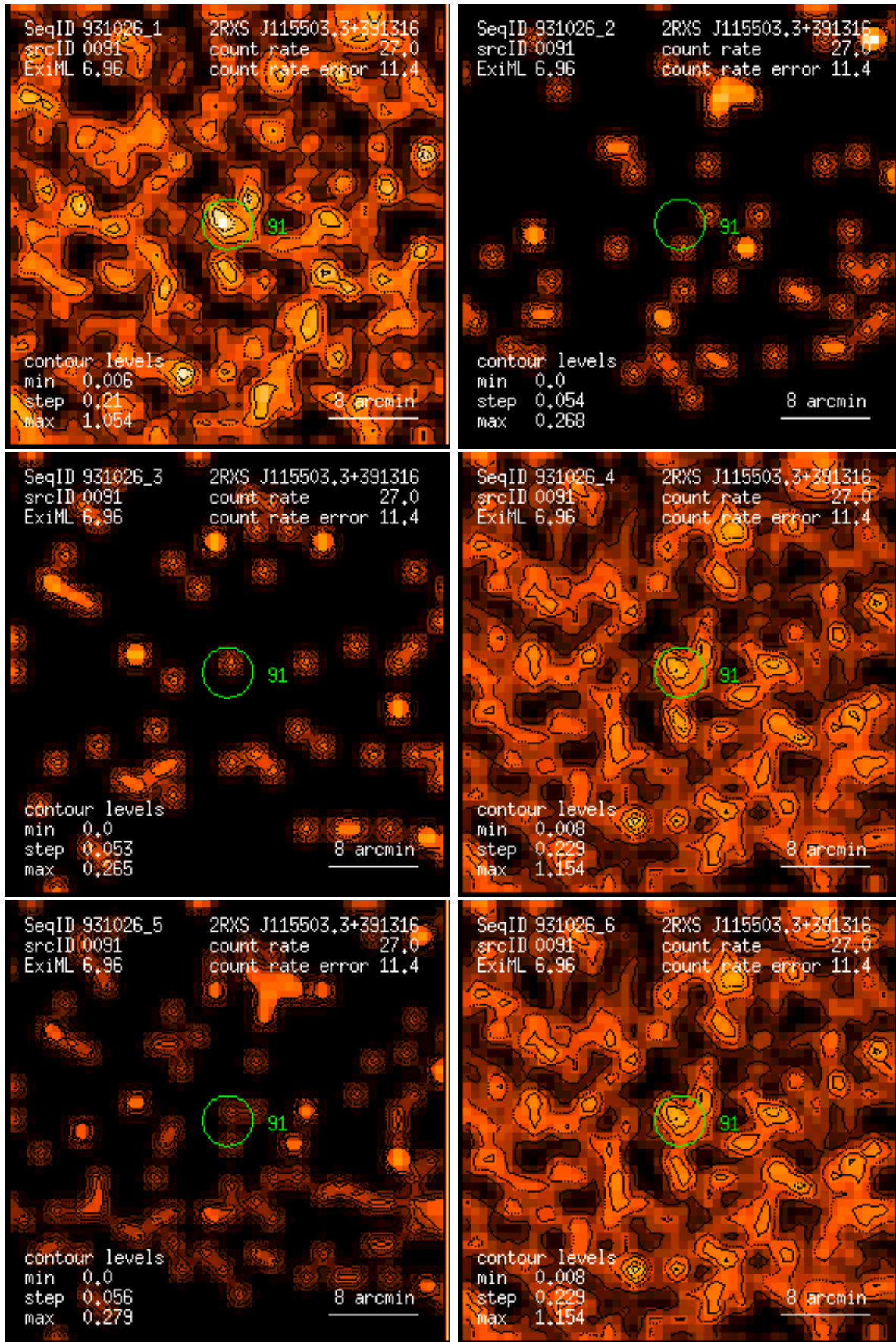
Figure 91: RASS 931026: detection 0091: band rate images, Gaussian filter: (1) PSPC channels 11 – 41, (2) 52 – 90, (3) 91 – 201, (4) 11 – 235, (5) 52 – 201, (6) 11 – 201. Broad band rates in counts/ks. Band rate contour levels in counts/ks/arcmin 2 .
