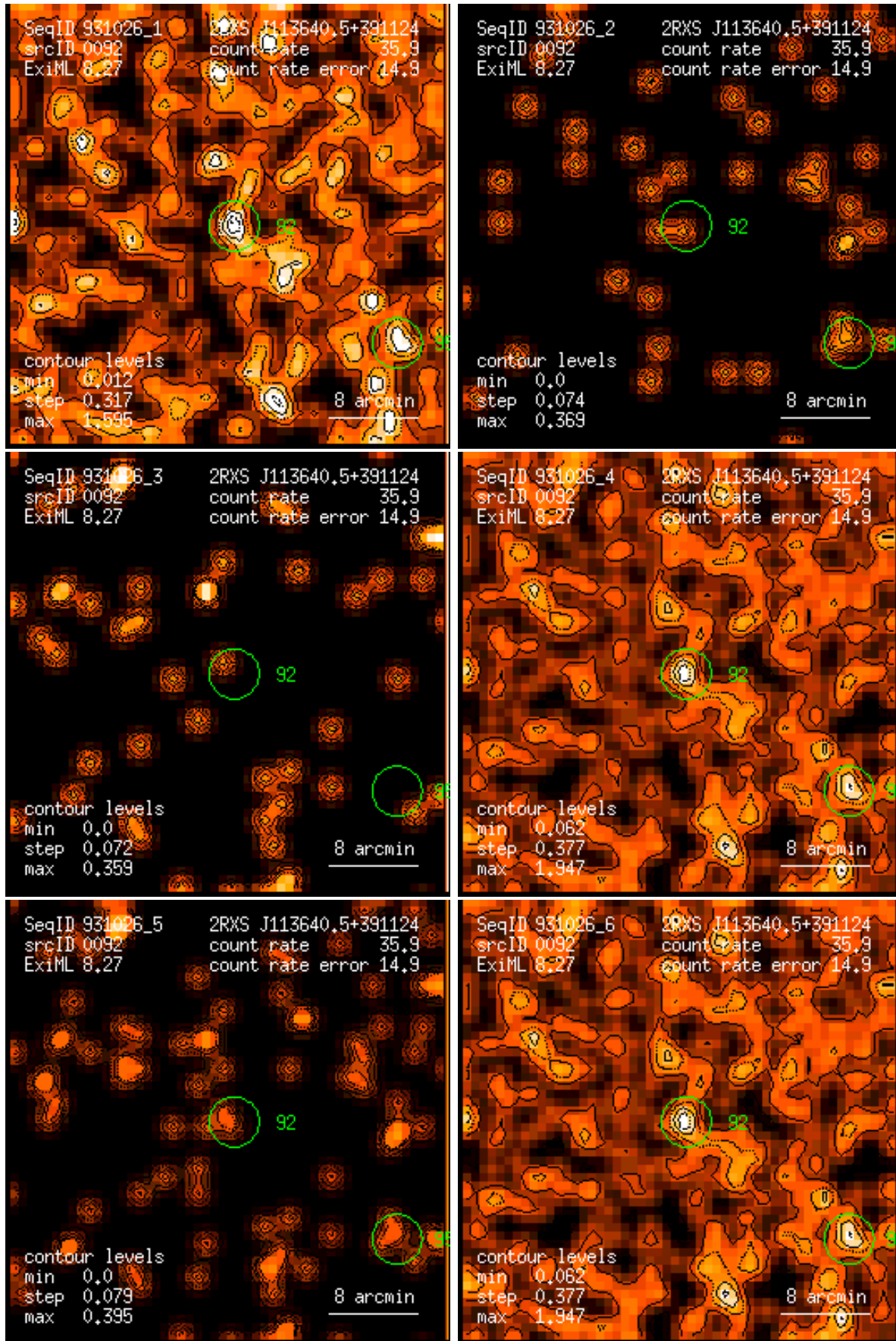
Figure 92: RASS 931026: detection 0092: band rate images, Gaussian filter: (1) PSPC channels 11 – 41, (2) 52 – 90, (3) 91 – 201, (4) 11 – 235, (5) 52 – 201, (6) 11 – 201. Broad band rates in counts/ks. Band rate contour levels in counts/ks/arcmin 2 .
