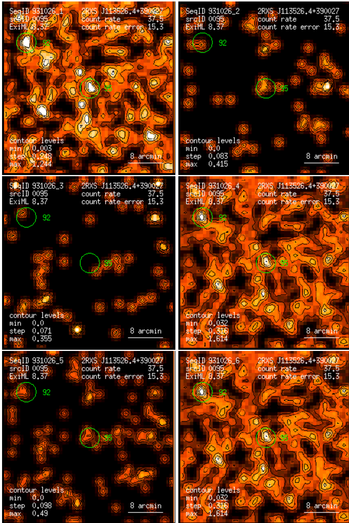
Figure 95: RASS 931026: detection 0095: band rate images, Gaussian filter: (1) PSPC channels 11 – 41, (2) 52 – 90, (3) 91 – 201, (4) 11 – 235, (5) 52 – 201, (6) 11 – 201. Broad band rates in counts/ks. Band rate contour levels in counts/ks/arcmin 2 .
