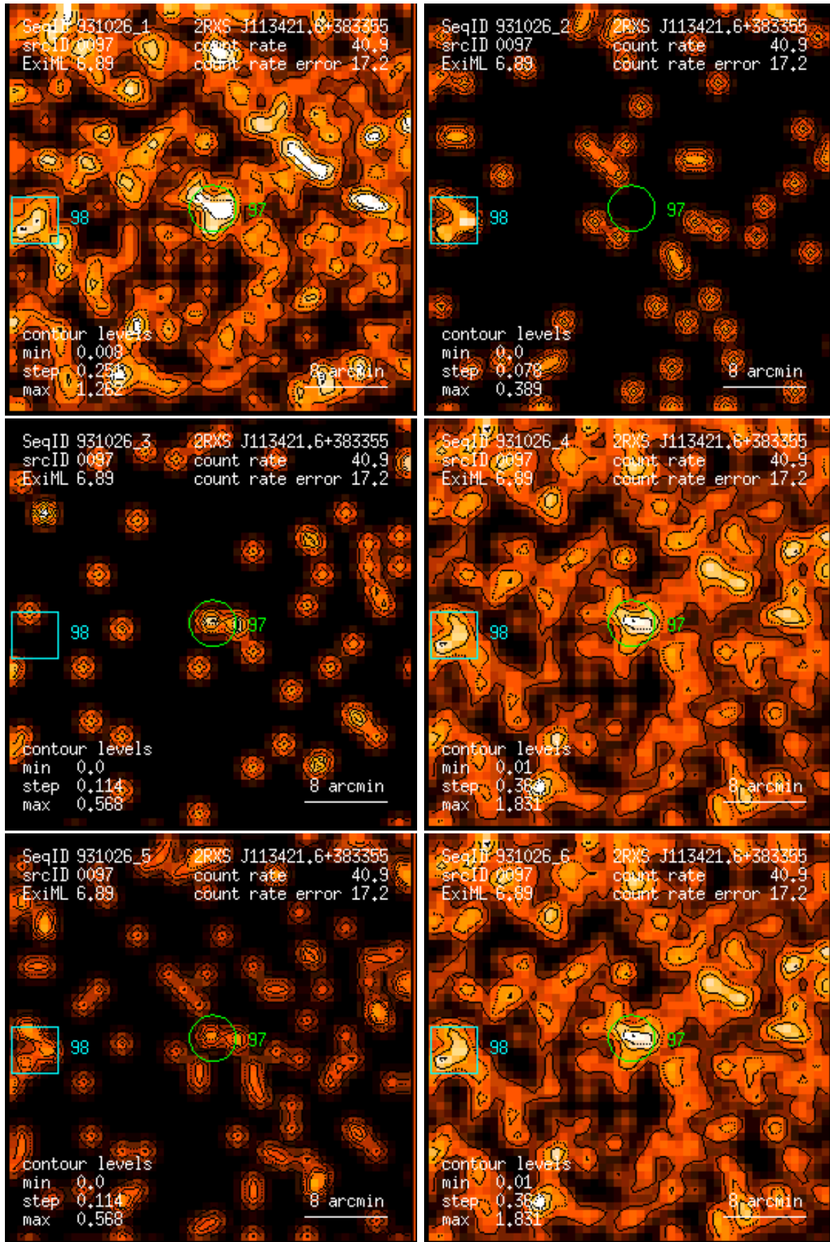
Figure 97: RASS 931026: detection 0097: band rate images, Gaussian filter: (1) PSPC channels 11 – 41, (2) 52 – 90, (3) 91 – 201, (4) 11 – 235, (5) 52 – 201, (6) 11 – 201. Broad band rates in counts/ks. Band rate contour levels in counts/ks/arcmin 2 .
