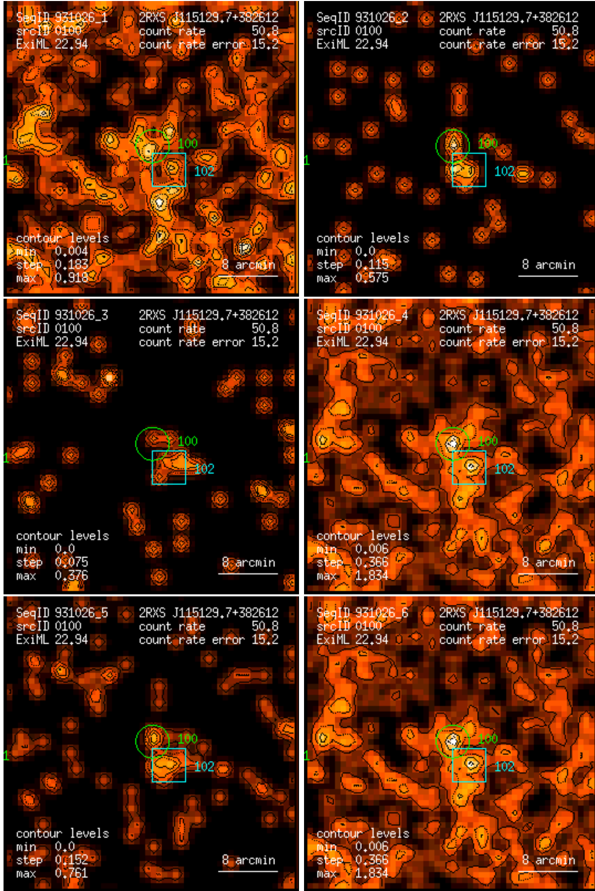
Figure 100: RASS 931026: detection 0100: band rate images, Gaussian filter: (1) PSPC channels 11 – 41, (2) 52 – 90, (3) 91 – 201, (4) 11 – 235, (5) 52 – 201, (6) 11 – 201. Broad band rates in counts/ks. Band rate contour levels in counts/ks/arcmin 2 .
