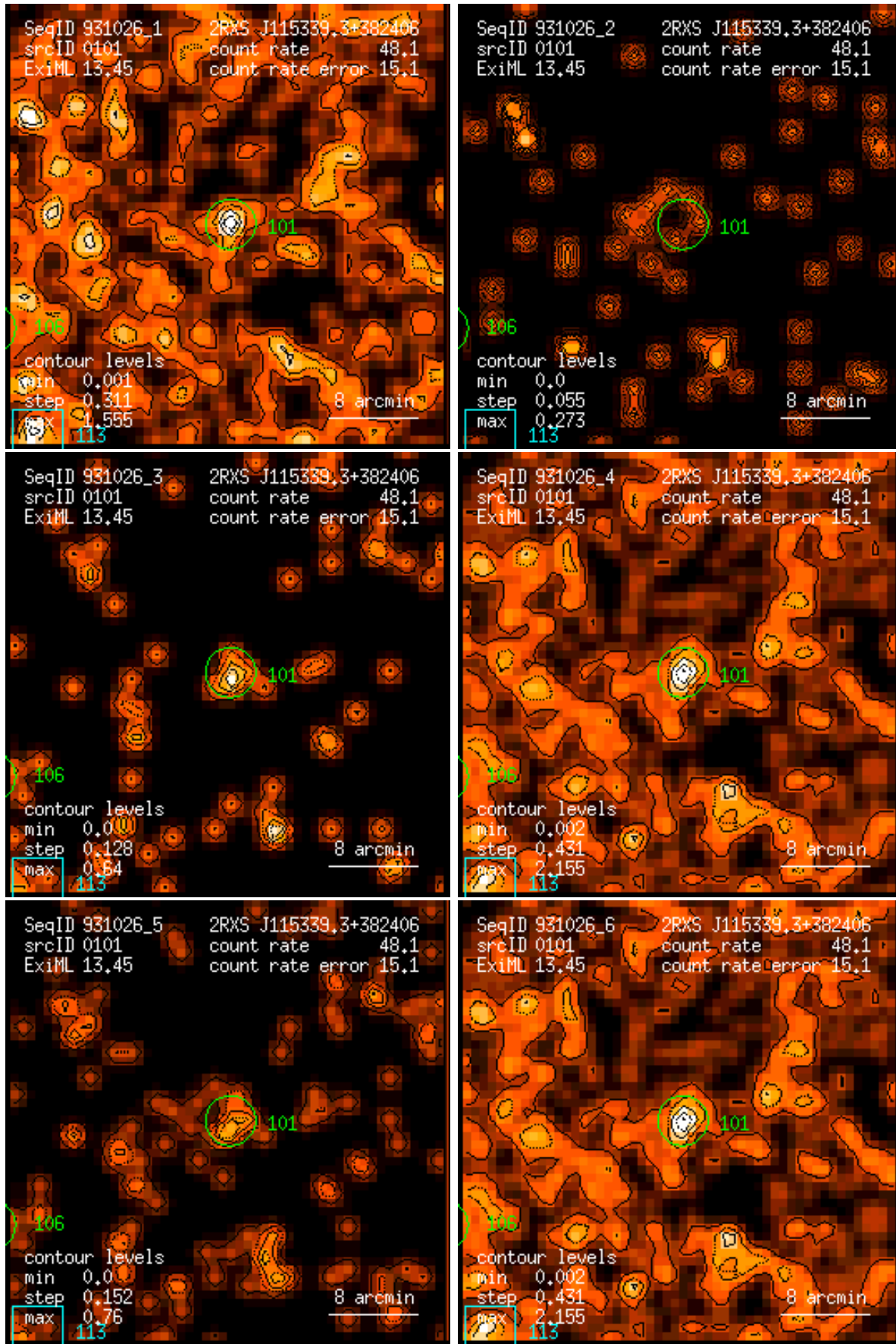
Figure 101: RASS 931026: detection 0101: band rate images, Gaussian filter: (1) PSPC channels 11 – 41, (2) 52 – 90, (3) 91 – 201, (4) 11 – 235, (5) 52 – 201, (6) 11 – 201. Broad band rates in counts/ks. Band rate contour levels in counts/ks/arcmin 2 .
