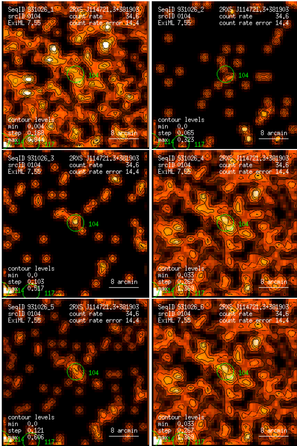
Figure 104: RASS 931026: detection 0104: band rate images, Gaussian filter: (1) PSPC channels 11 – 41, (2) 52 – 90, (3) 91 – 201, (4) 11 – 235, (5) 52 – 201, (6) 11 – 201. Broad band rates in counts/ks. Band rate contour levels in counts/ks/arcmin 2 .
