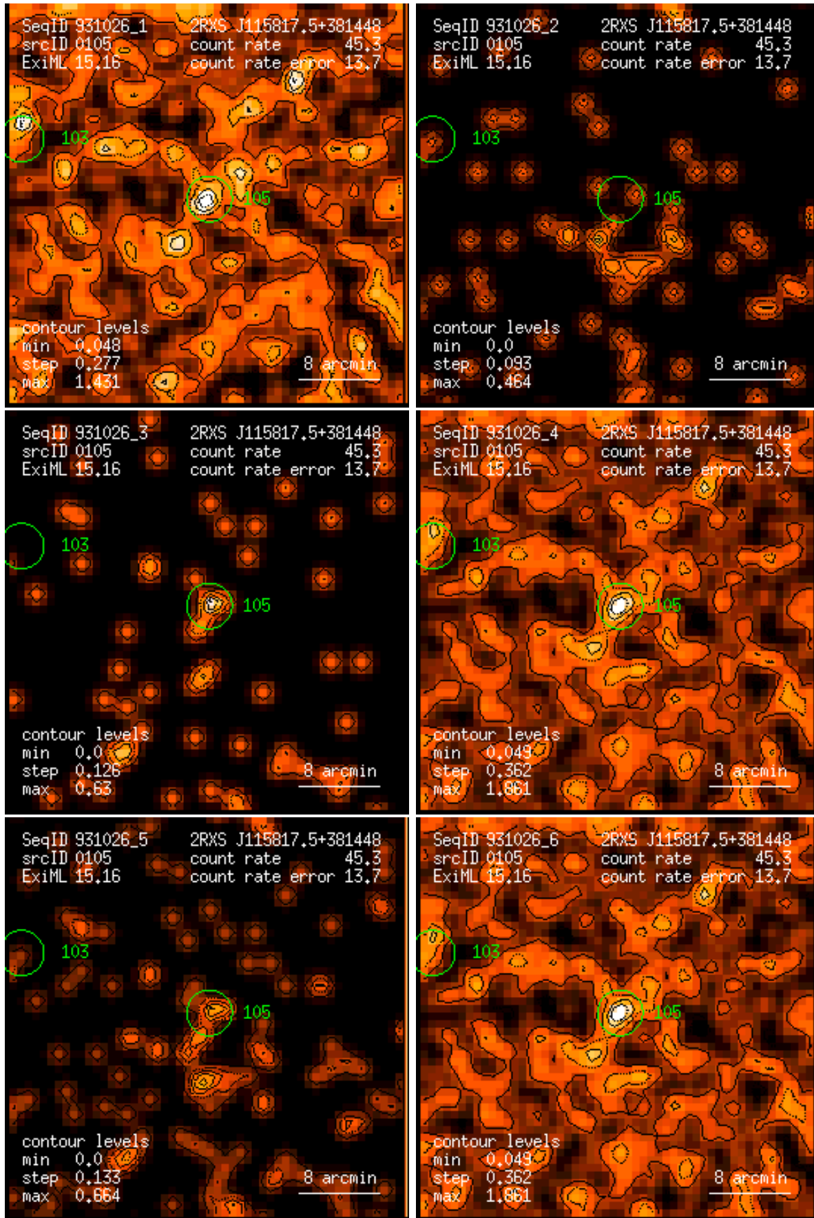
Figure 105: RASS 931026: detection 0105: band rate images, Gaussian filter: (1) PSPC channels 11 – 41, (2) 52 – 90, (3) 91 – 201, (4) 11 – 235, (5) 52 – 201, (6) 11 – 201. Broad band rates in counts/ks. Band rate contour levels in counts/ks/arcmin 2 .
