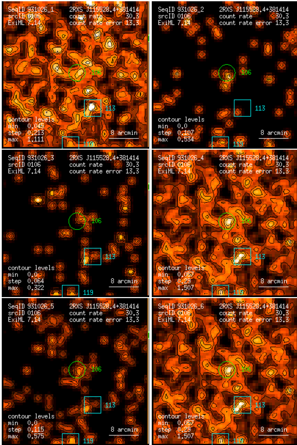
Figure 106: RASS 931026: detection 0106: band rate images, Gaussian filter: (1) PSPC channels 11 – 41, (2) 52 – 90, (3) 91 – 201, (4) 11 – 235, (5) 52 – 201, (6) 11 – 201. Broad band rates in counts/ks. Band rate contour levels in counts/ks/arcmin 2 .
