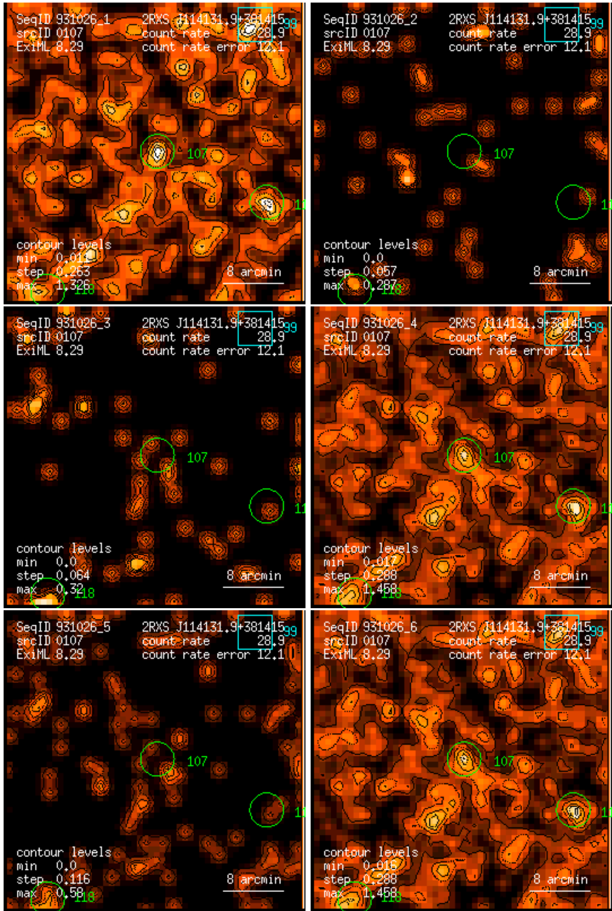
Figure 107: RASS 931026: detection 0107: band rate images, Gaussian filter: (1) PSPC channels 11 – 41, (2) 52 – 90, (3) 91 – 201, (4) 11 – 235, (5) 52 – 201, (6) 11 – 201. Broad band rates in counts/ks. Band rate contour levels in counts/ks/arcmin 2 .
