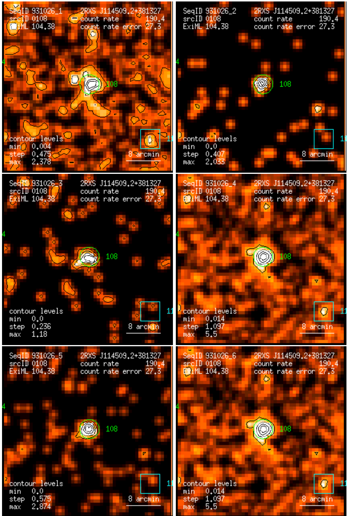
Figure 108: RASS 931026: detection 0108: band rate images, Gaussian filter: (1) PSPC channels 11 – 41, (2) 52 – 90, (3) 91 – 201, (4) 11 – 235, (5) 52 – 201, (6) 11 – 201. Broad band rates in counts/ks. Band rate contour levels in counts/ks/arcmin 2 .
