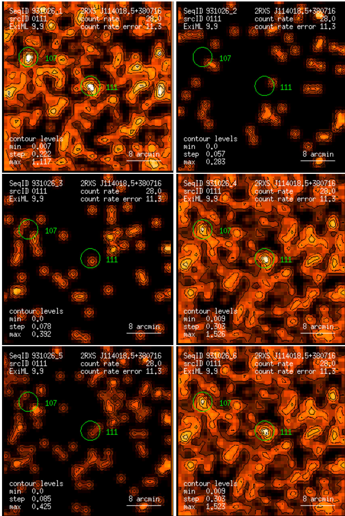
Figure 111: RASS 931026: detection 0111: band rate images, Gaussian filter: (1) PSPC channels 11 – 41, (2) 52 – 90, (3) 91 – 201, (4) 11 – 235, (5) 52 – 201, (6) 11 – 201. Broad band rates in counts/ks. Band rate contour levels in counts/ks/arcmin 2 .
