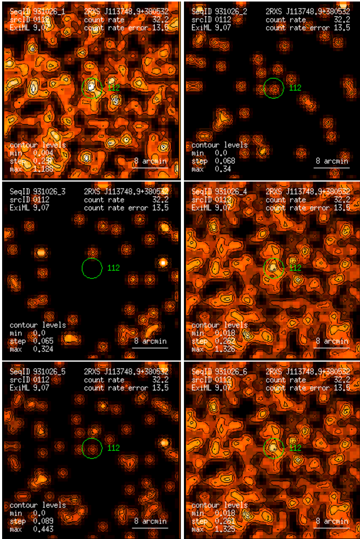
Figure 112: RASS 931026: detection 0112: band rate images, Gaussian filter: (1) PSPC channels 11 – 41, (2) 52 – 90, (3) 91 – 201, (4) 11 – 235, (5) 52 – 201, (6) 11 – 201. Broad band rates in counts/ks. Band rate contour levels in counts/ks/arcmin 2 .
