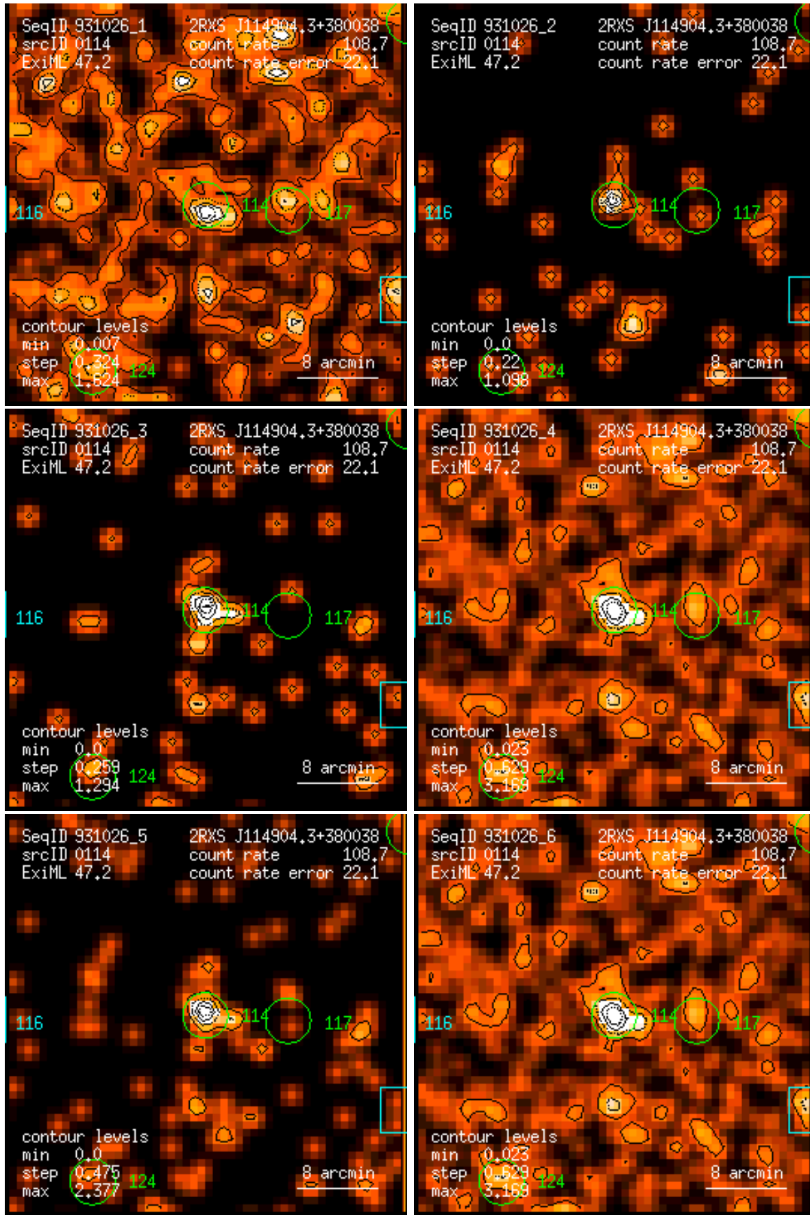
Figure 114: RASS 931026: detection 0114: band rate images, Gaussian filter: (1) PSPC channels 11 – 41, (2) 52 – 90, (3) 91 – 201, (4) 11 – 235, (5) 52 – 201, (6) 11 – 201. Broad band rates in counts/ks. Band rate contour levels in counts/ks/arcmin 2 .
