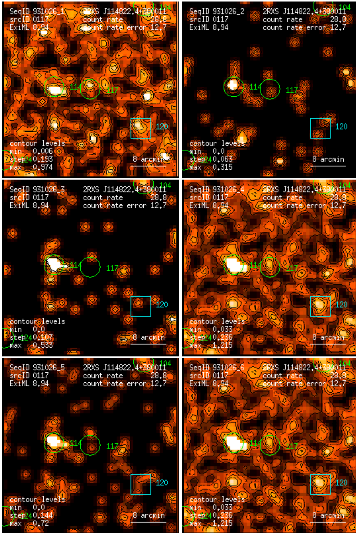
Figure 117: RASS 931026: detection 0117: band rate images, Gaussian filter: (1) PSPC channels 11 – 41, (2) 52 – 90, (3) 91 – 201, (4) 11 – 235, (5) 52 – 201, (6) 11 – 201. Broad band rates in counts/ks. Band rate contour levels in counts/ks/arcmin 2 .
