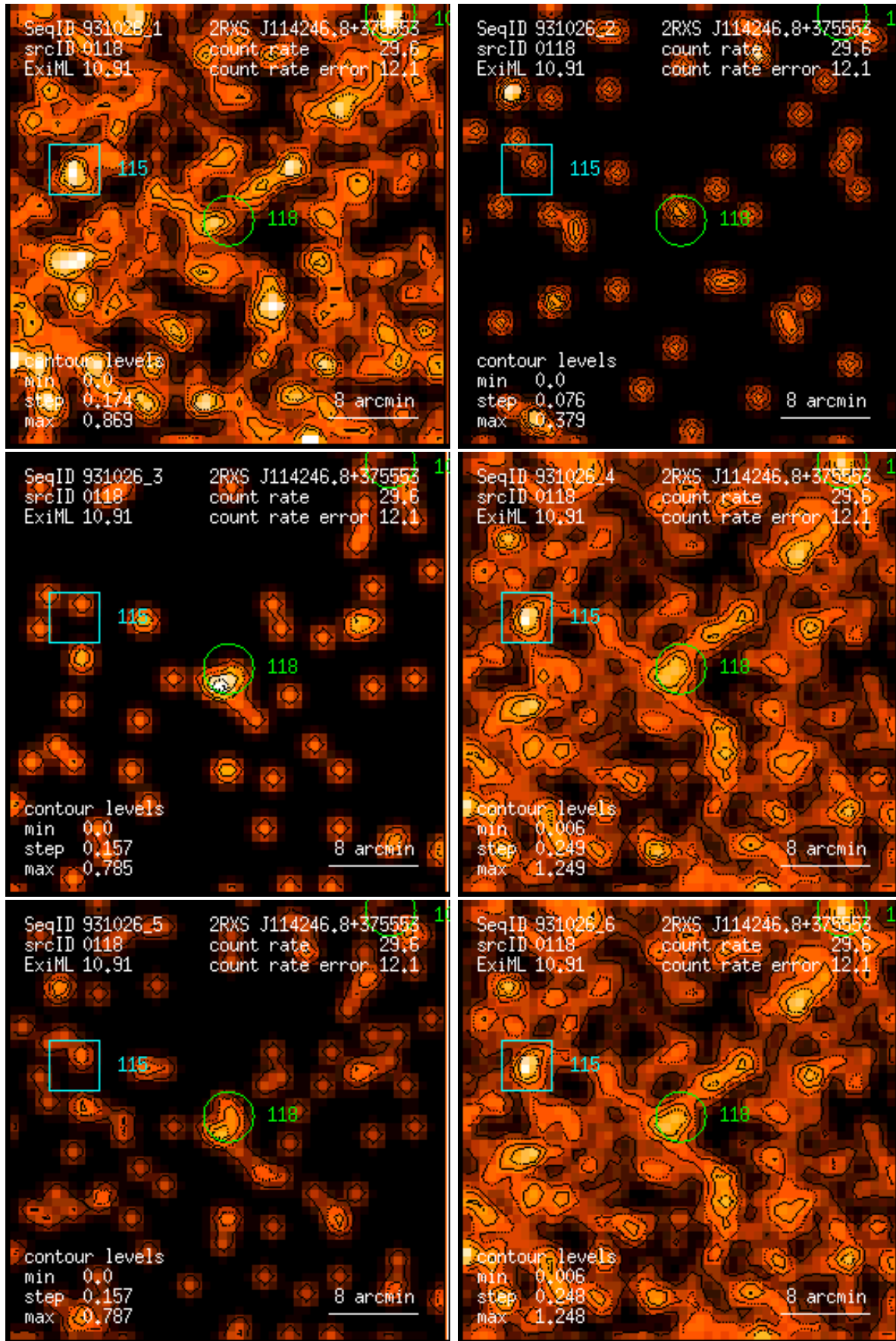
Figure 118: RASS 931026: detection 0118: band rate images, Gaussian filter: (1) PSPC channels 11 – 41, (2) 52 – 90, (3) 91 – 201, (4) 11 – 235, (5) 52 – 201, (6) 11 – 201. Broad band rates in counts/ks. Band rate contour levels in counts/ks/arcmin 2 .
