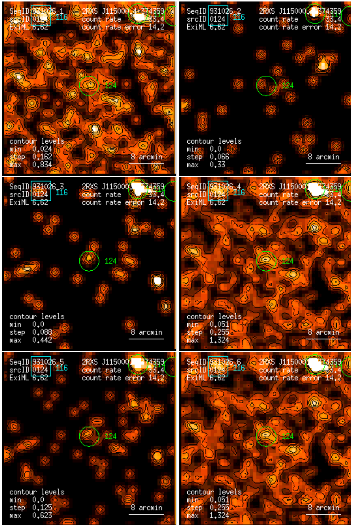
Figure 124: RASS 931026: detection 0124: band rate images, Gaussian filter: (1) PSPC channels 11 – 41, (2) 52 – 90, (3) 91 – 201, (4) 11 – 235, (5) 52 – 201, (6) 11 – 201. Broad band rates in counts/ks. Band rate contour levels in counts/ks/arcmin 2 .
