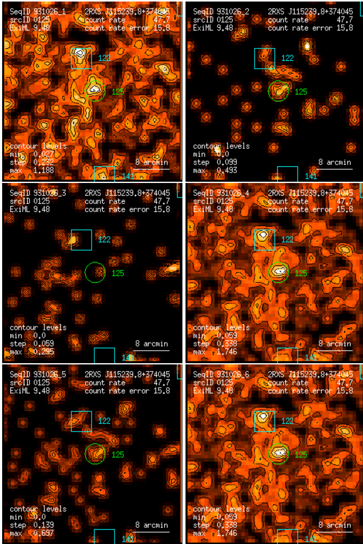
Figure 125: RASS 931026: detection 0125: band rate images, Gaussian filter: (1) PSPC channels 11 – 41, (2) 52 – 90, (3) 91 – 201, (4) 11 – 235, (5) 52 – 201, (6) 11 – 201. Broad band rates in counts/ks. Band rate contour levels in counts/ks/arcmin 2 .
