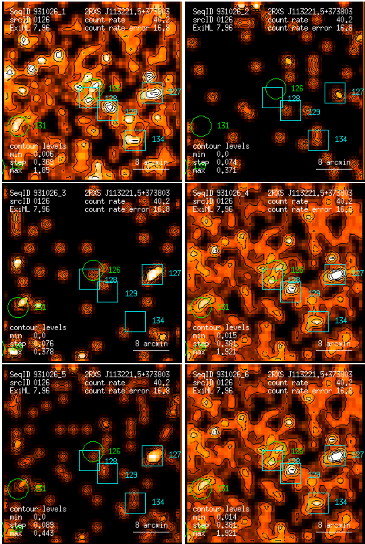
Figure 126: RASS 931026: detection 0126: band rate images, Gaussian filter: (1) PSPC channels 11 – 41, (2) 52 – 90, (3) 91 – 201, (4) 11 – 235, (5) 52 – 201, (6) 11 – 201. Broad band rates in counts/ks. Band rate contour levels in counts/ks/arcmin 2 .
